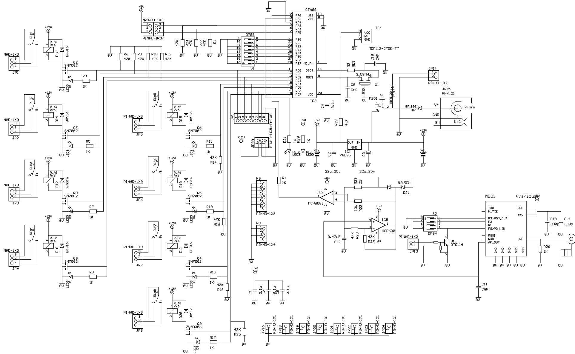
Figure 11: Schematic of CTA88 Decoder application board for SHX1R / UHX1R / FPX3R Receiver
