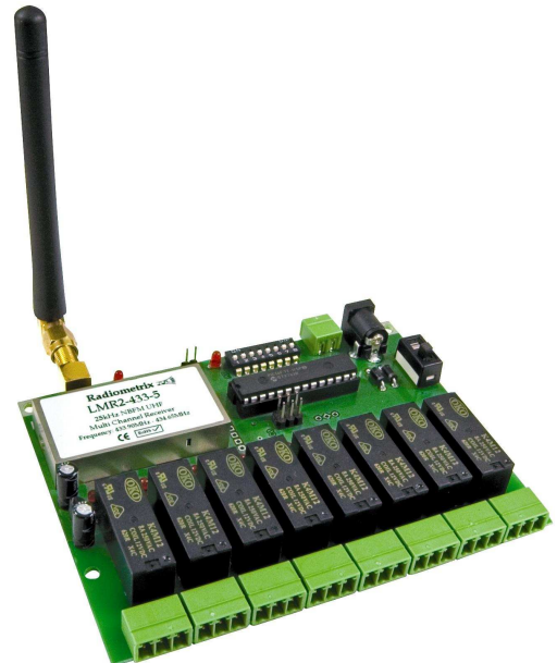
Figure 1: CTA88 RX application board
