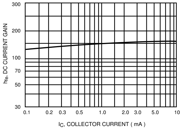
Figure 9. Current Gain
