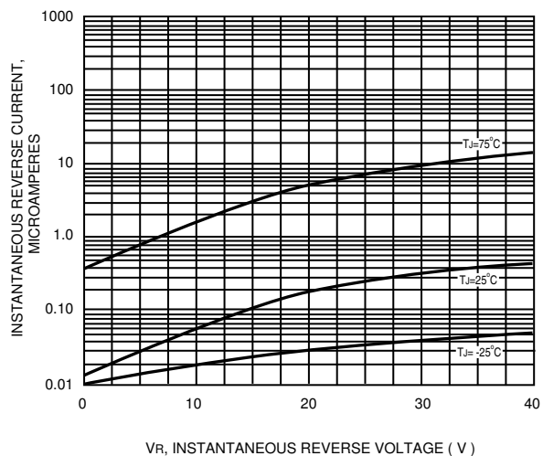
FIG. 4 - REVERSE CHARACTERISTICS
