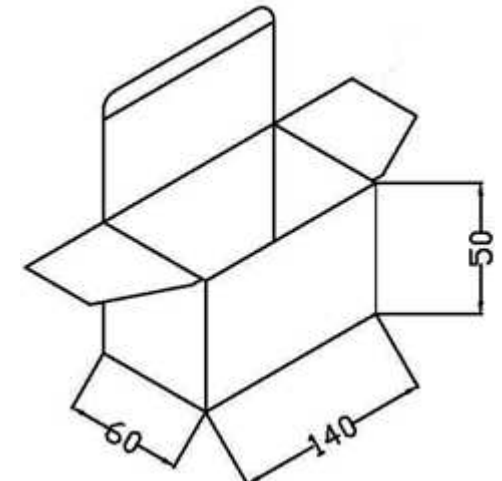
White Inner Box Dimensions
