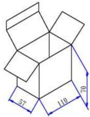
Inner Box Dimensions
