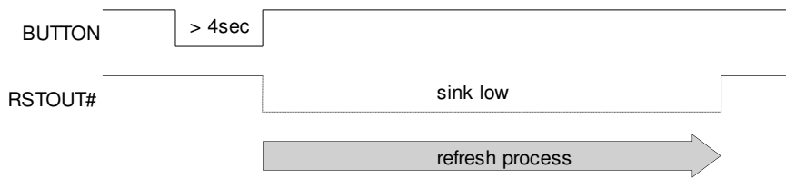
Figure 7.4.3.1 BUTTON illustrator with RSTOUT# sink low
