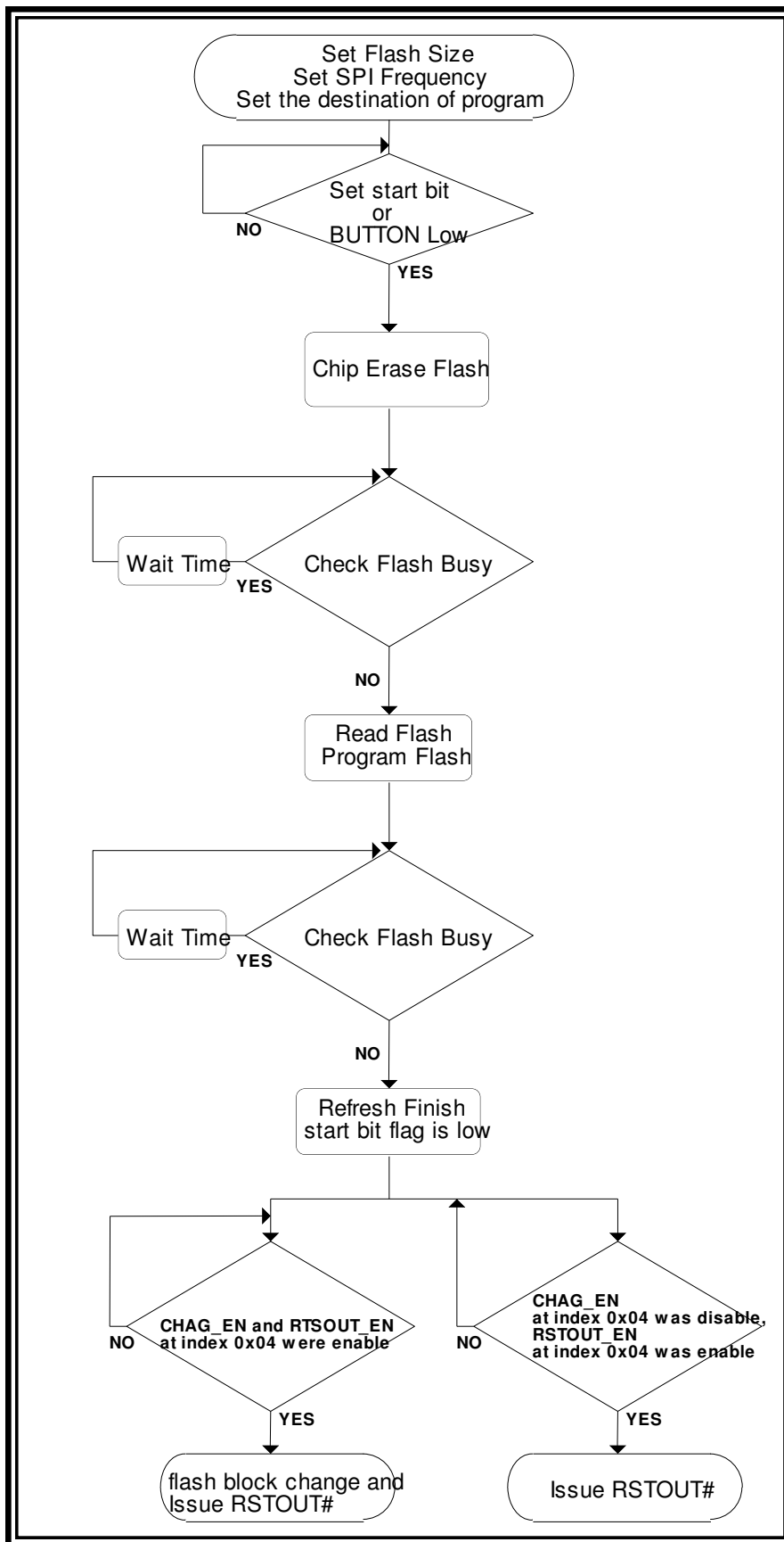
Figure 7.6.1 describe RSTOUT's status and flash block status after WDT happened timeout.
