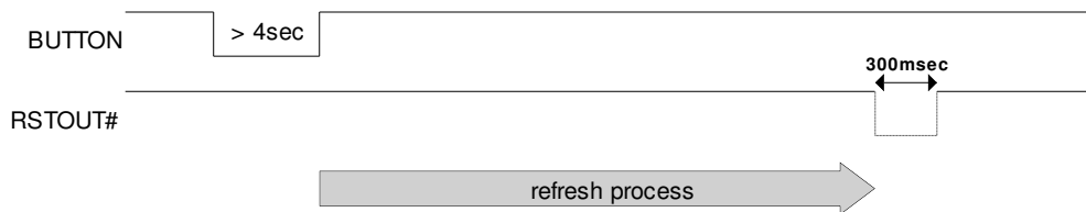
Figure 7.4.3.2 BUTTON illustrator with RSTOUT# low pulse
