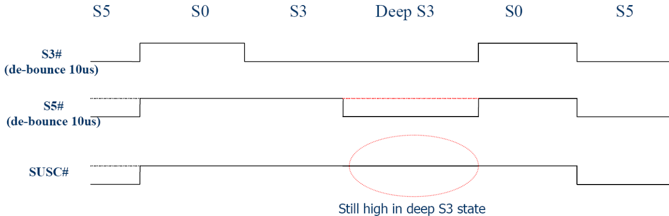
Figure 25 SUSC# timing
