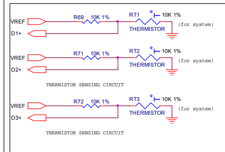
Temperature Sensing
