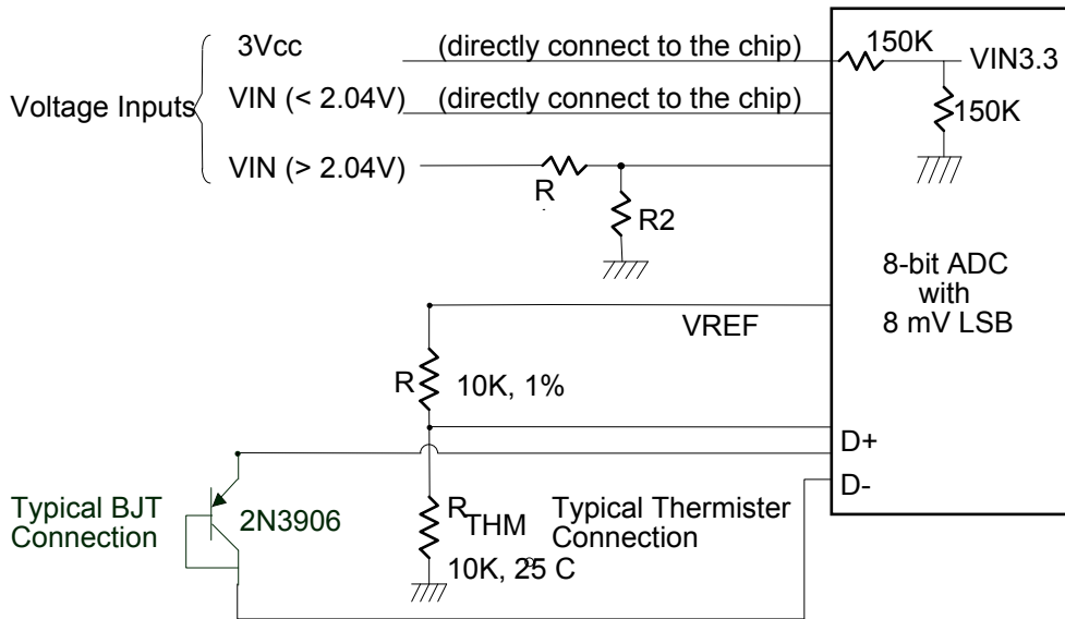
Figure 1. Hardware monitor configuration
