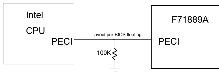
INTEL PECI Typical Application
