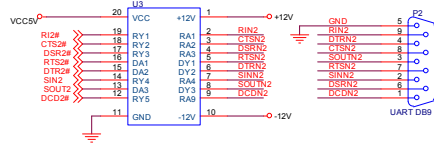
UART 2 PORT INTERFACE
