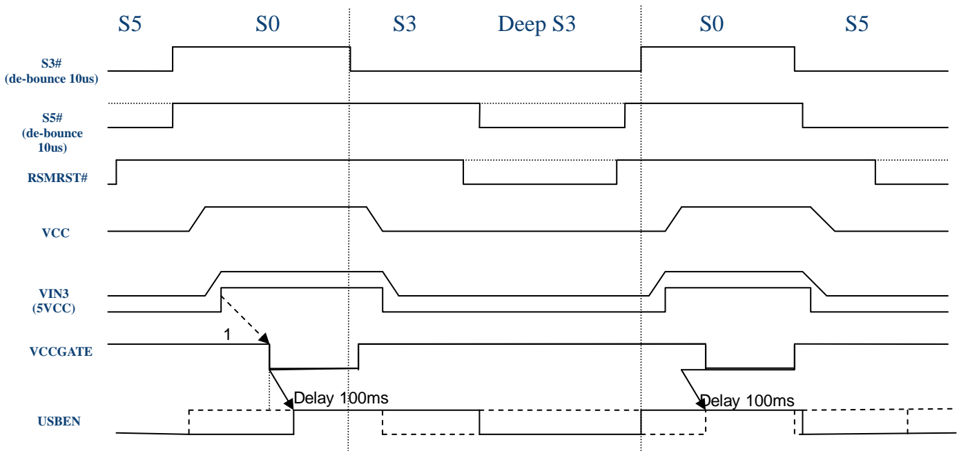
Figure 24 VCCGATE &amp; USBEN timing
