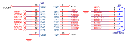
UART 1 PORT INTERFACE
