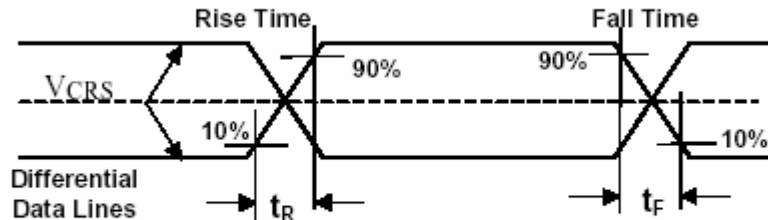
USB timing
