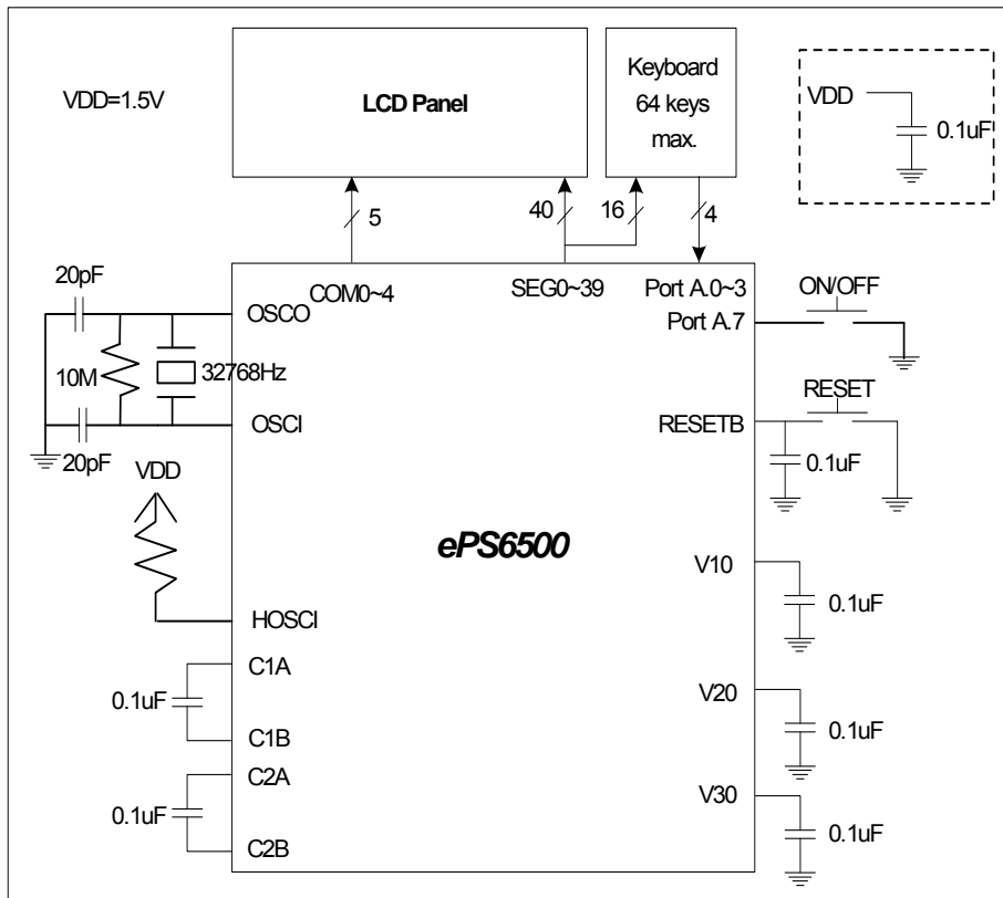
Figure 11-1 VDD=1.5V Application Circuit Diagram
