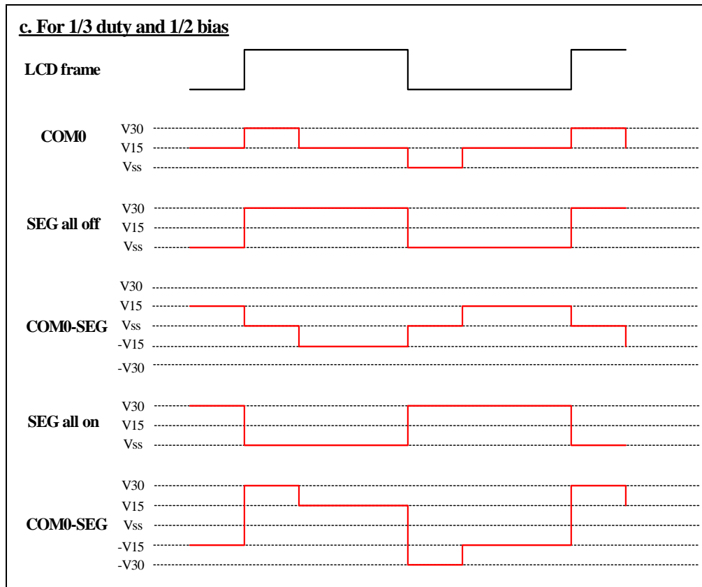
Figure 8-17 LCD COM & SEG Waveform for 1/3 Duty and 1/2 Bias
