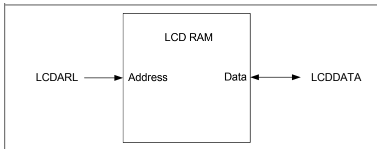
Figure 8-9 LCDDATA Register Access through LCD RAM
