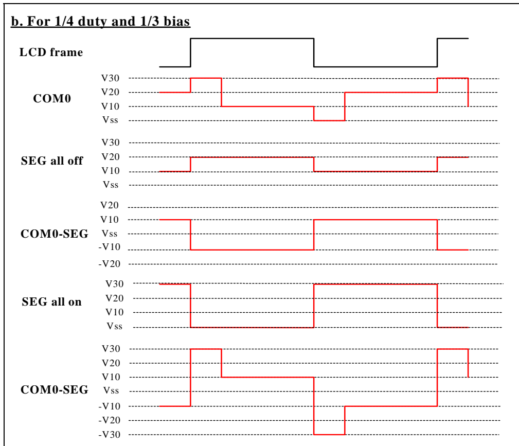
Figure 8-16 LCD COM & SEG Waveform for 1/4 Duty and 1/3 Bias
