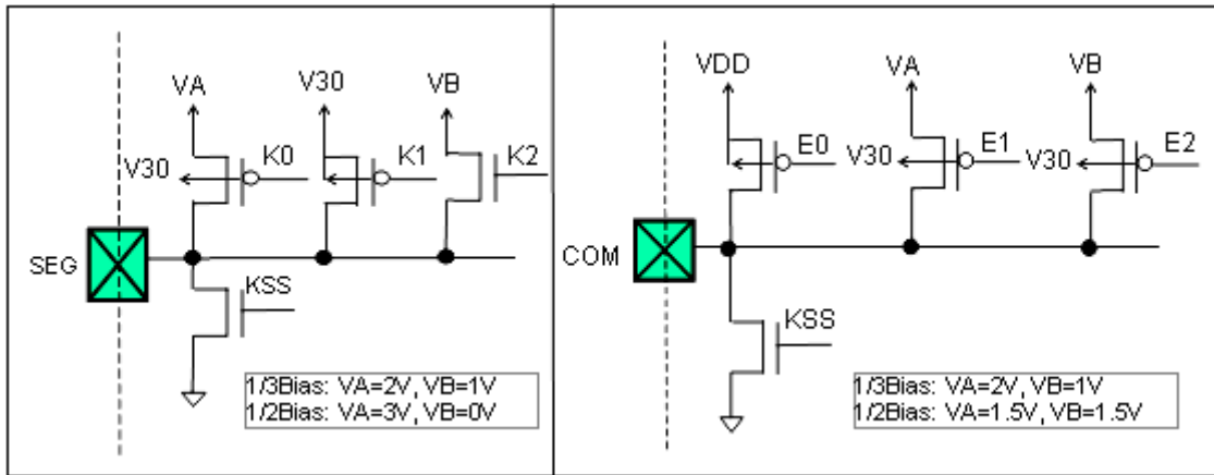
Figure 10-1g General SEG & COM Share Pin Type Circuit Diagram
