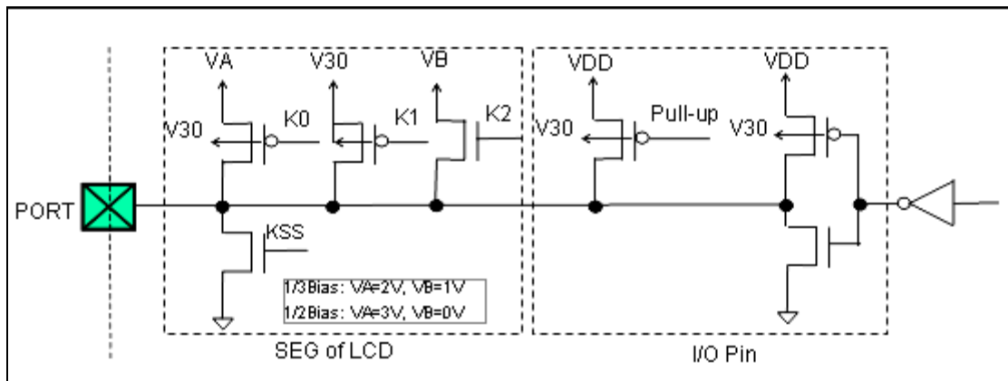
Figure 10-1f SEG & I/O Share Pin Type Circuit Diagram
