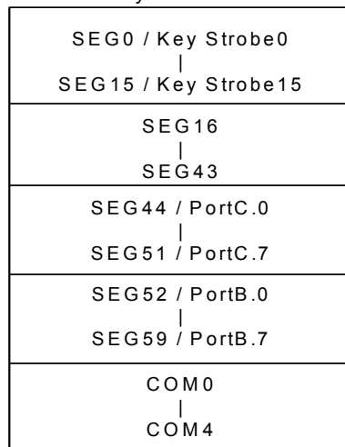
Figure 8-8b LCD Pin Configuration
