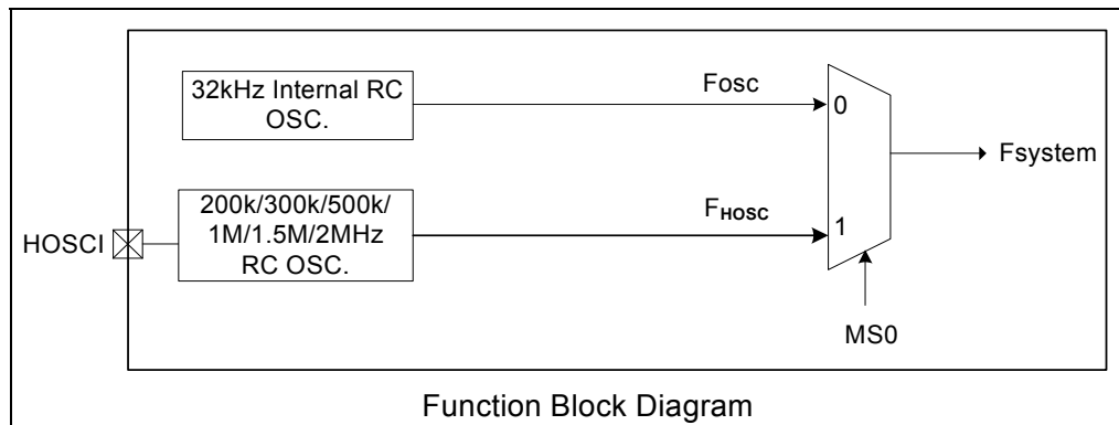
Figure 7-3 Oscillator System Function Block Diagram
