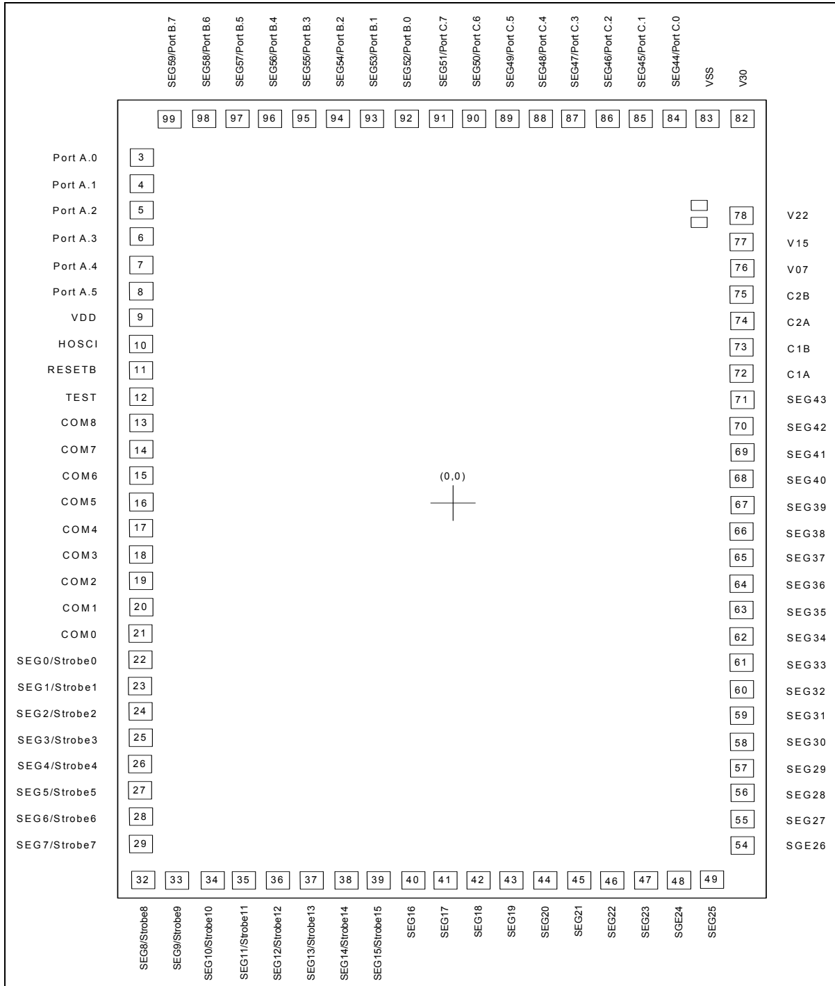
Figure 13-1 ePS6001 88 Pin-Out
