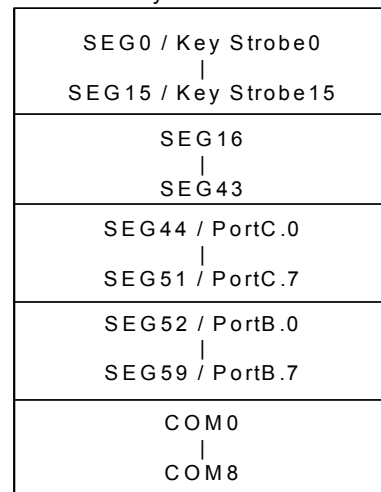
Figure 8-8b LCD Pin Configuration
