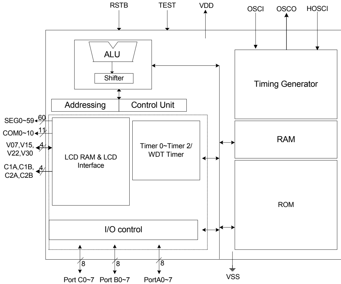
Figure 3-1 ePS5005 Block Diagram
