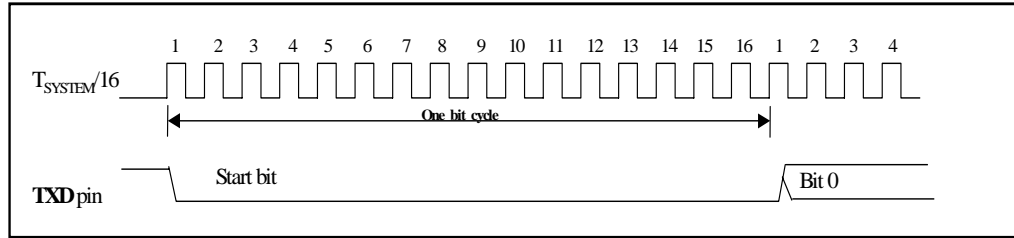
Fig. 8-9 UART Transmit Counter Timing
