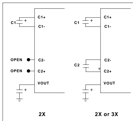
Fig. 8-23 External Capacitors
