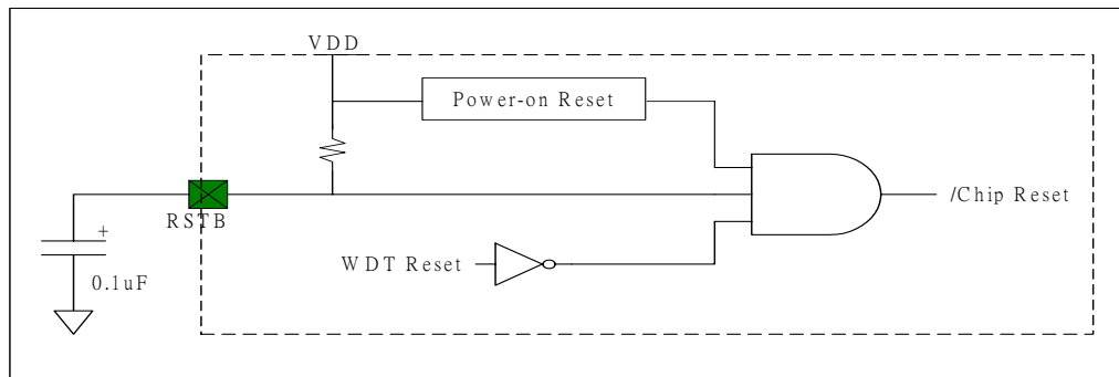
Fig 7-1 On-chip RESET Circuit
