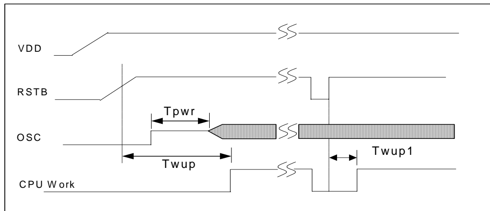
Fig 7-2 Power-up and RESET Timing
