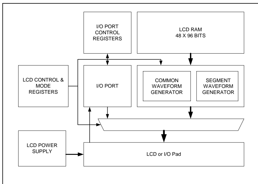
Fig. 8-21 Function Block Diagram
