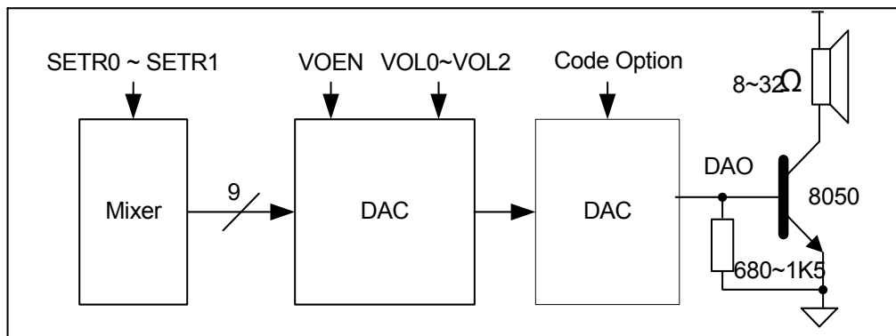
Figure 8-29 DAC Function Block Diagram
