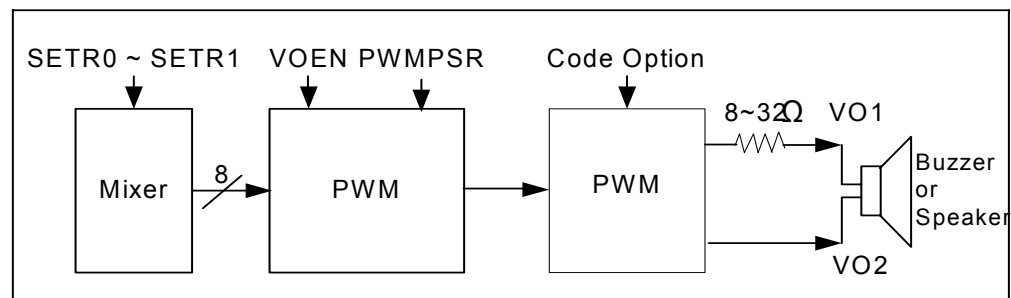
Figure 8-28 PWM Function Block Diagram
