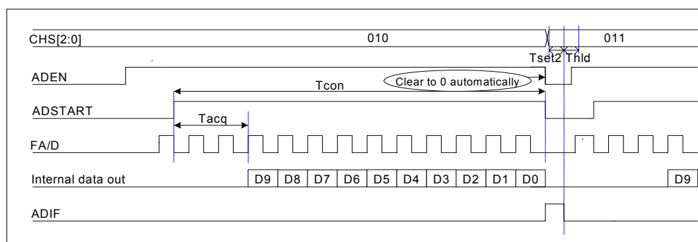
Figure 8-16 A/D Converter General Application Timing Diagram
