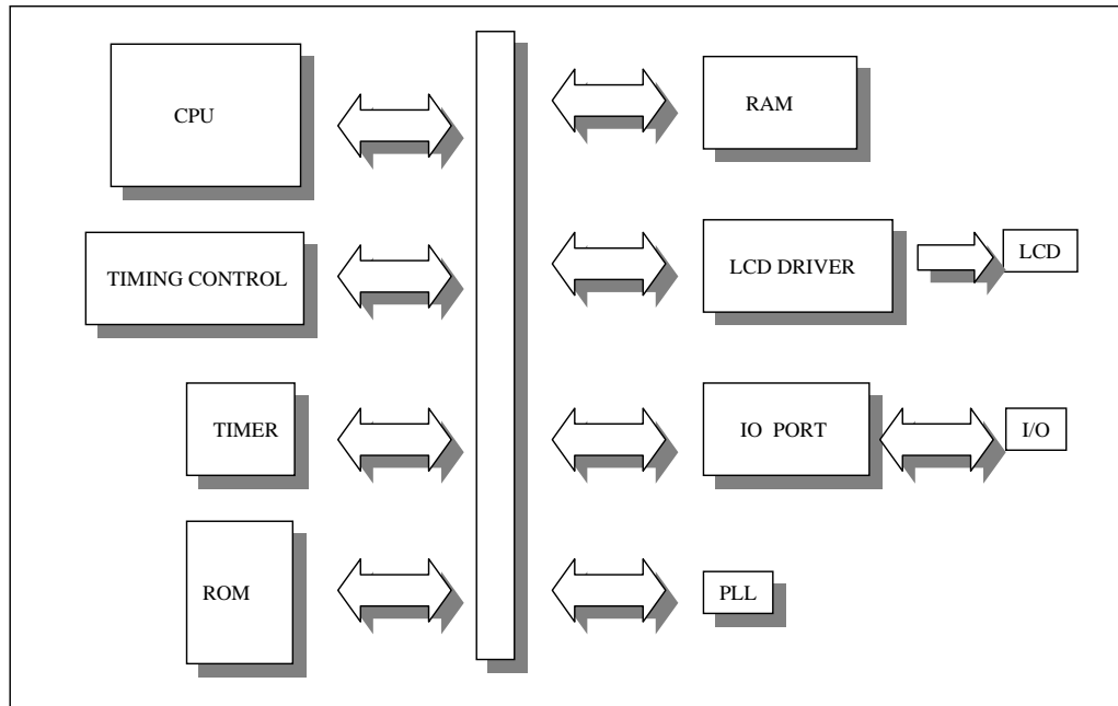
Fig. 5-1 System Overview Block Diagram
