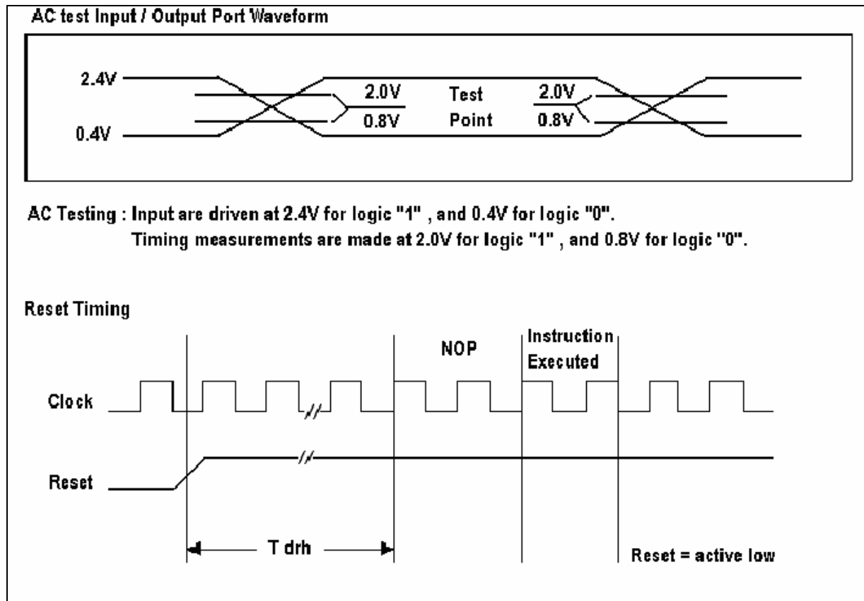
Fig. 10 AC Timing
