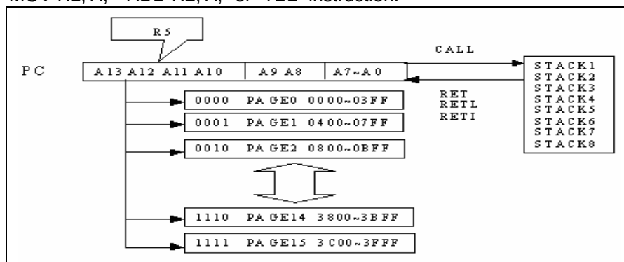
Fig. 6-1 Program Counter Organization
