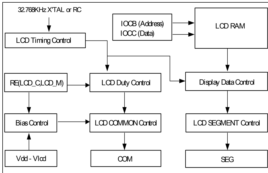
Fig. 6-10 LCD Driver Control Block
