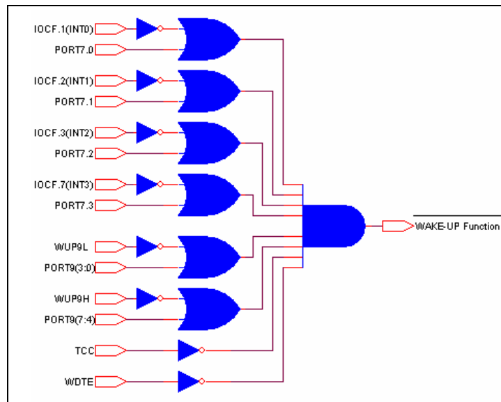
Fig. 6-4 Wake-up Function and Control Signal
