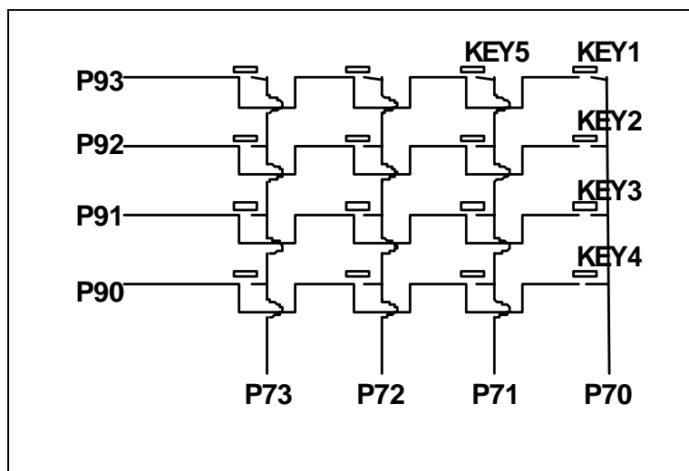
Fig. 6-5 Key Scans Circuit
