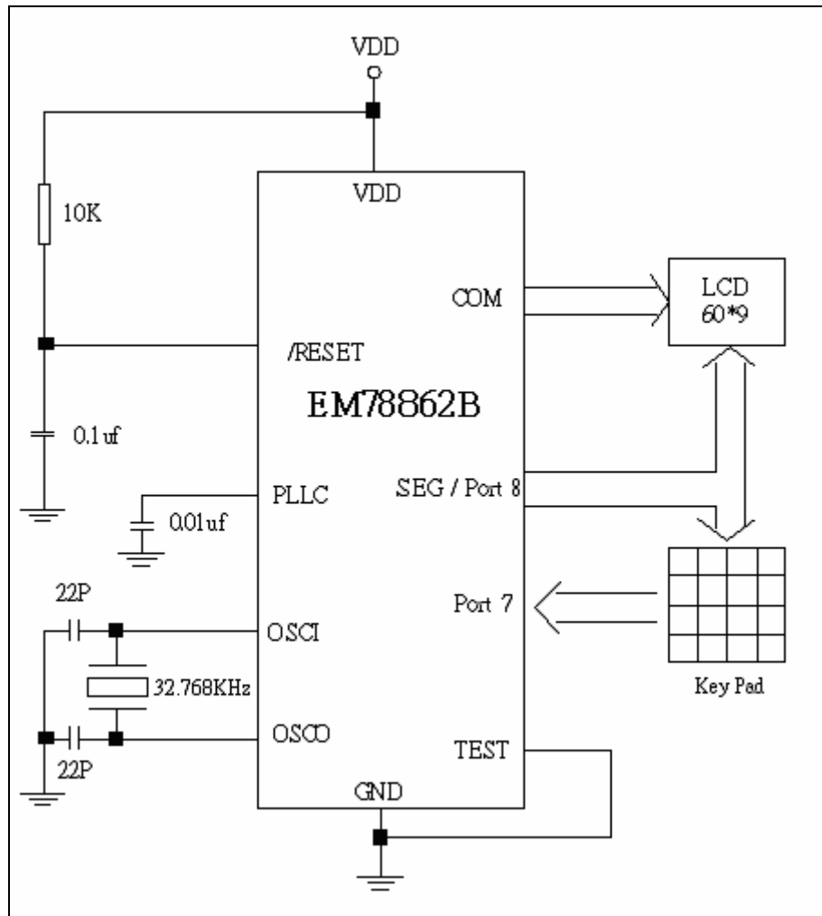
Fig. 11-1 Application with Crystal Mode
