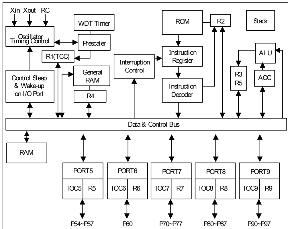
Fig. 5-2 System Functional Block Diagram
