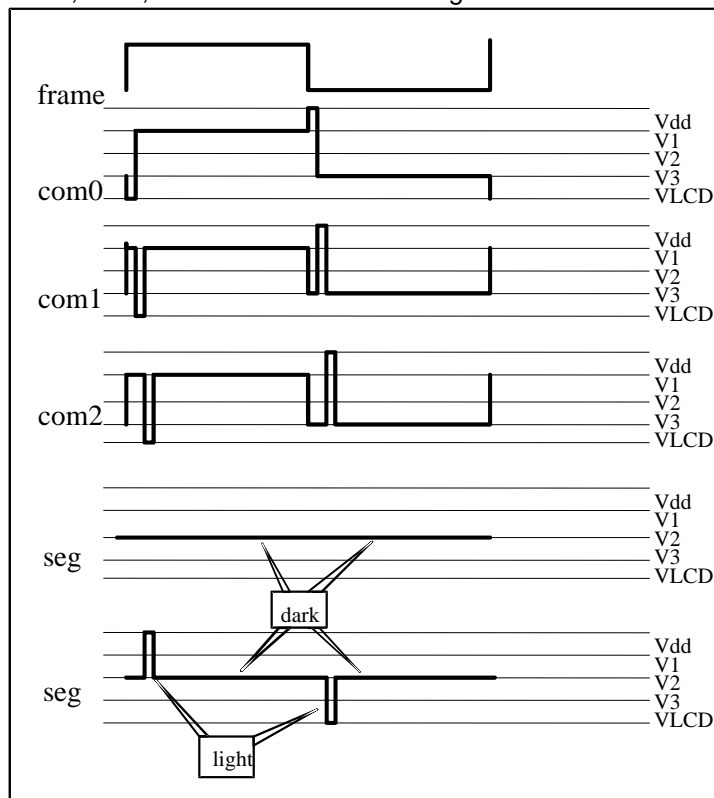
Fig. 6-11 LCD Waveform 1/4 Bias
