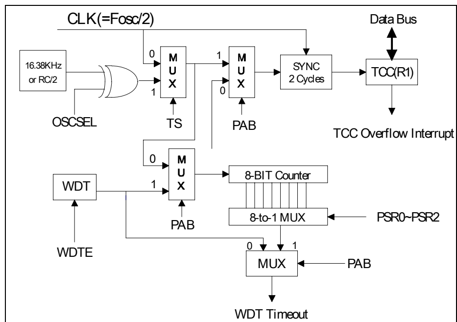
Fig. 6-7 TCC WDT Block Diagram
