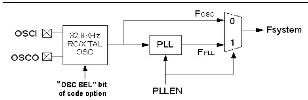
Fig. 6-9 Oscillator and PLL Function Block.
