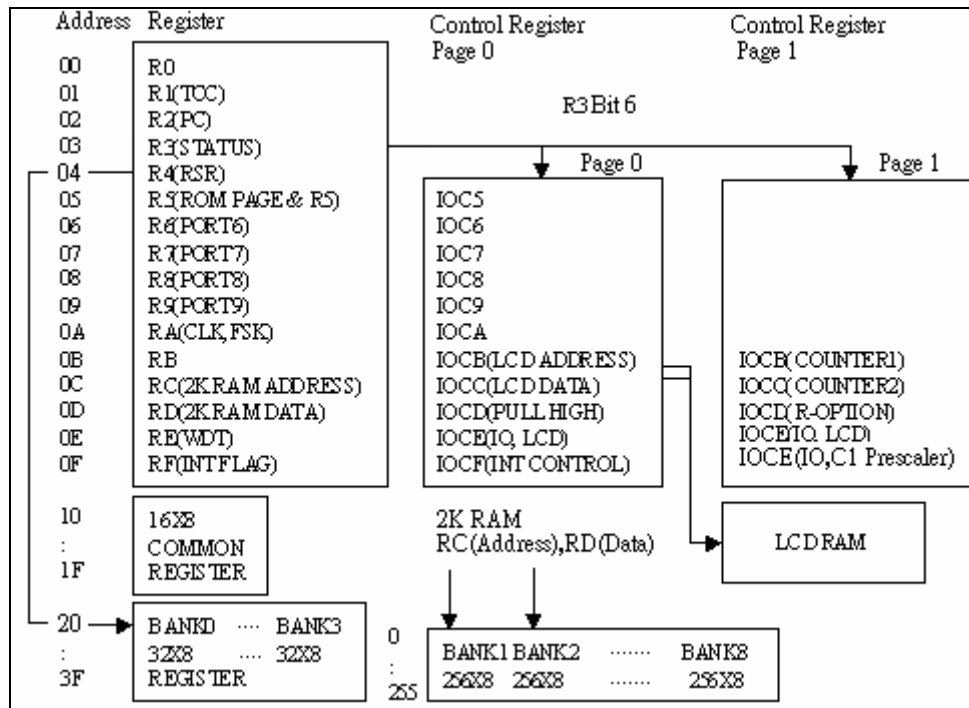
Fig. 6-2 Data Memory Configuration
