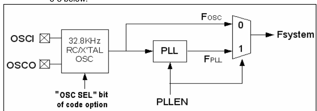
Fig. 6-3 The Relation between 32.768KHz and 3.579MHz
