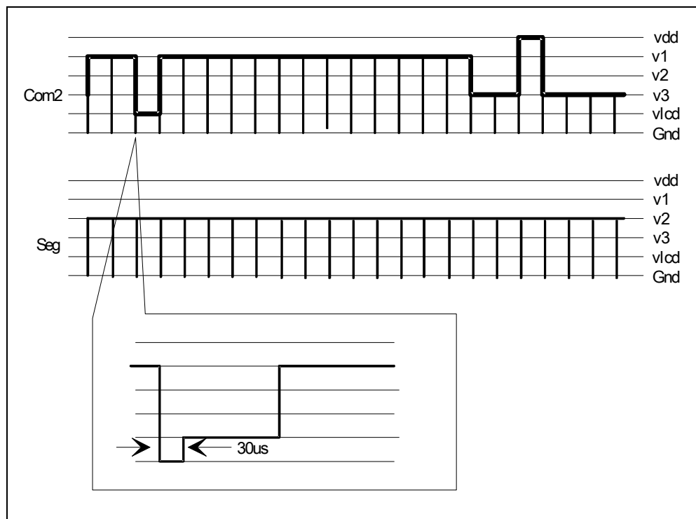
Fig. 6-6 Key Scan Signal
