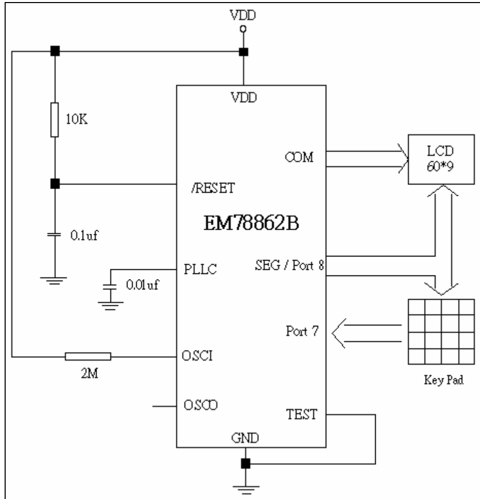
Fig. 11-2 Application with RC Mode
