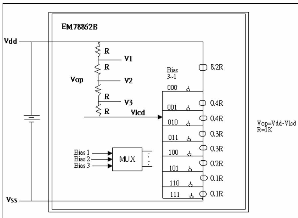
Fig. 6-12 LCD Bias Circuit
