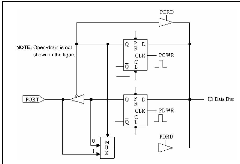
Fig. 6-8 Port 5, Port 6, Port 7, & Port 8 I/O Port and I/O Control Register Circuit
