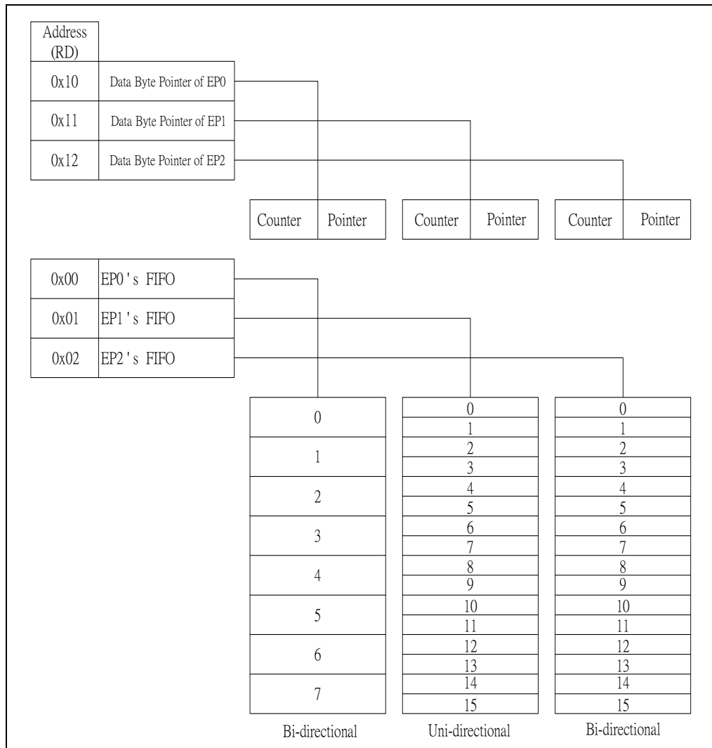
Figure 7-4 Functional Map Diagram of USB Application FIFO
