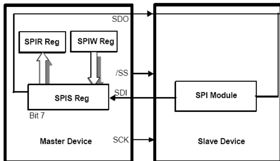
Figure 7-5a SPI Master/Slave Communication
