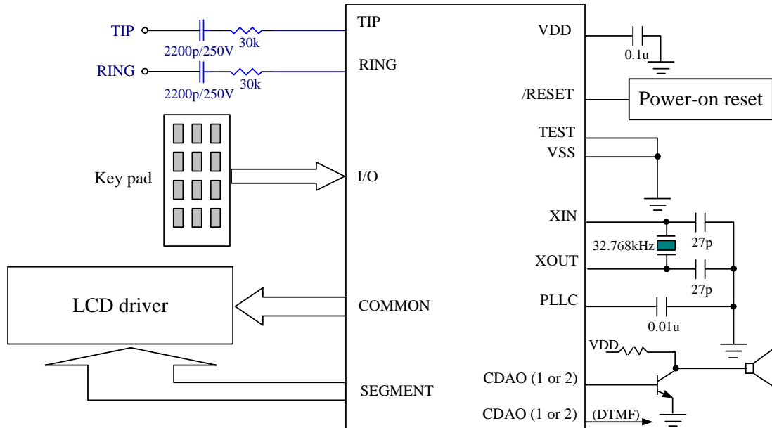
Fig 10-1 Application Circuit
