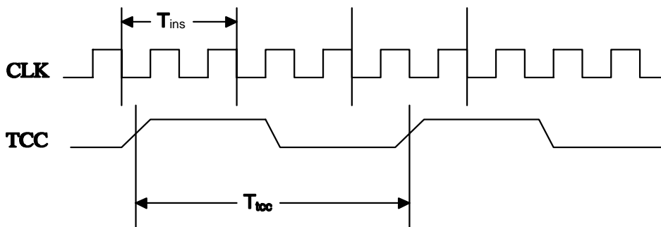
Fig 9-1 AC Timing
