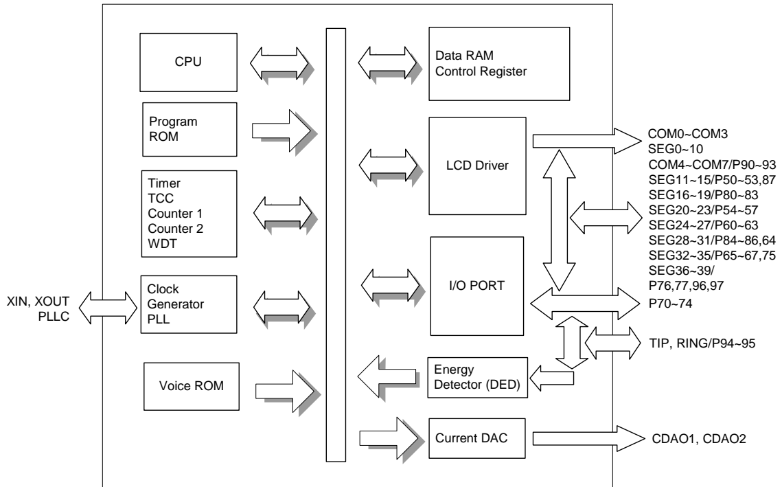
Fig 5-1 Block Diagram
