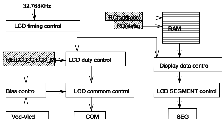
Fig 7-9 LCD Driver Control
