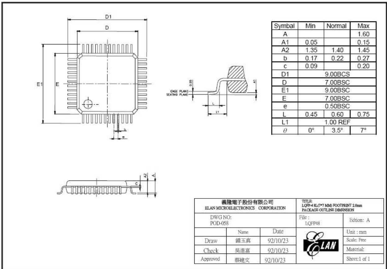
LQFP-48 dimension
