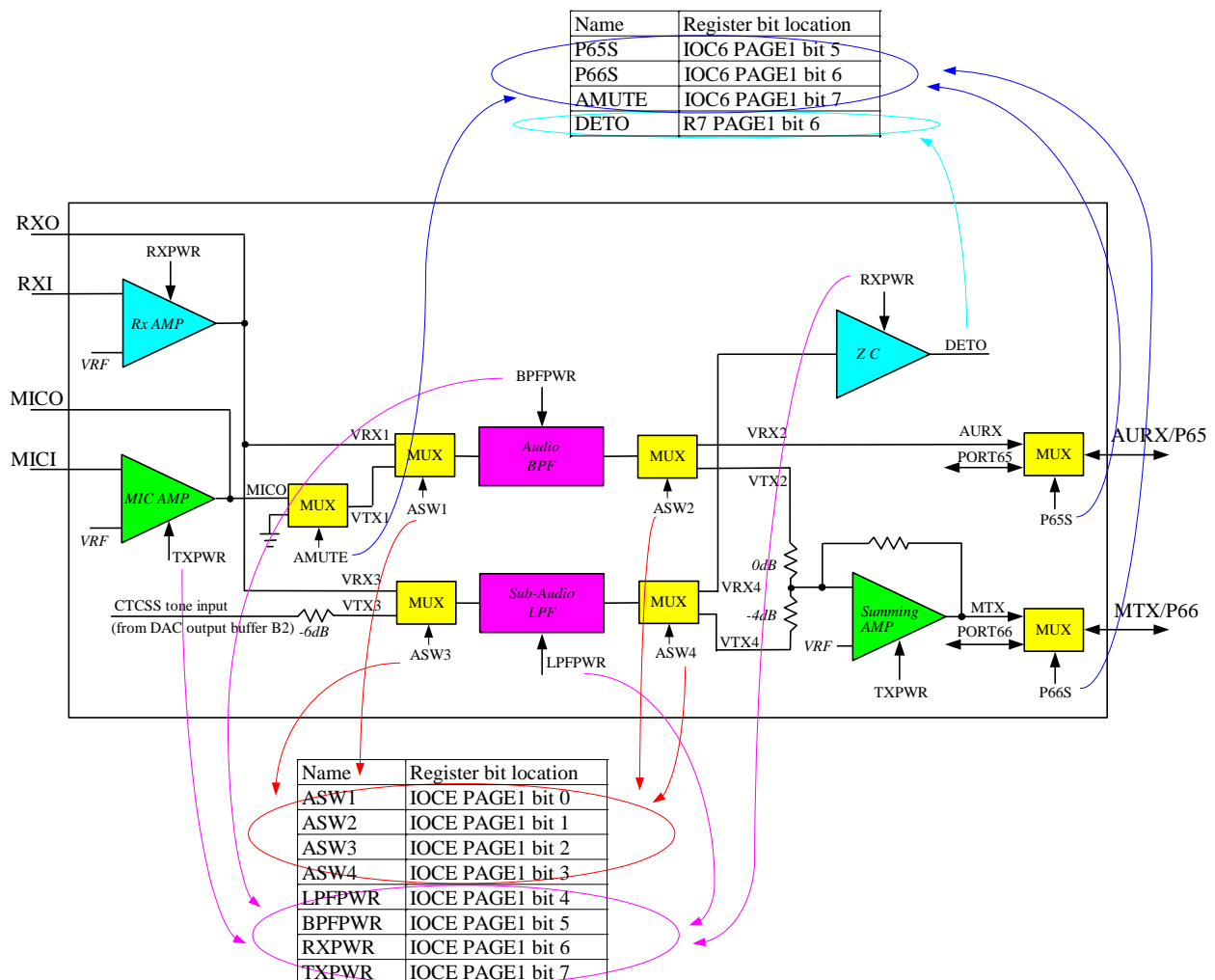
Fig.14 CTCSS block
