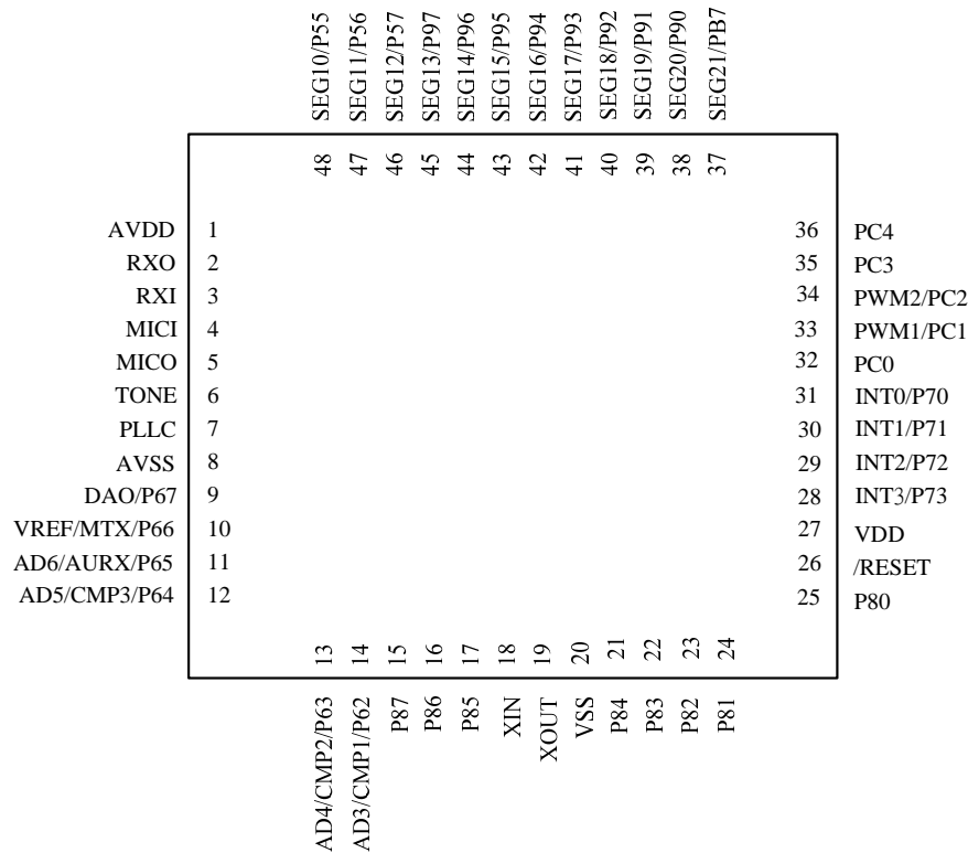
48-pin LQFP
