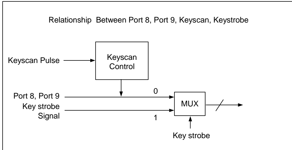
Fig. 23 Keyscan, Key strobe and Segments
