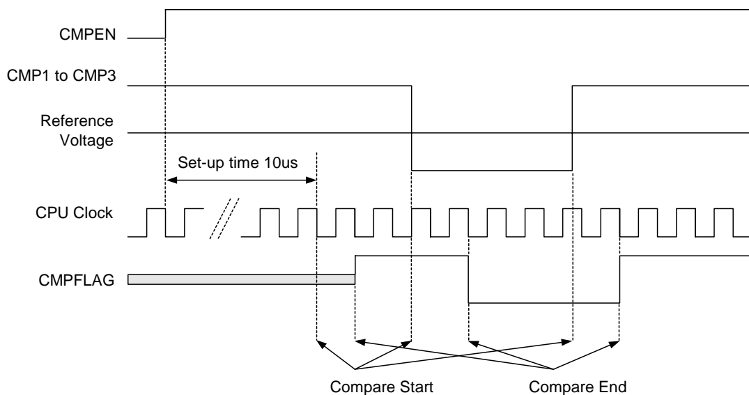
Fig. 20 Comparator Timing
