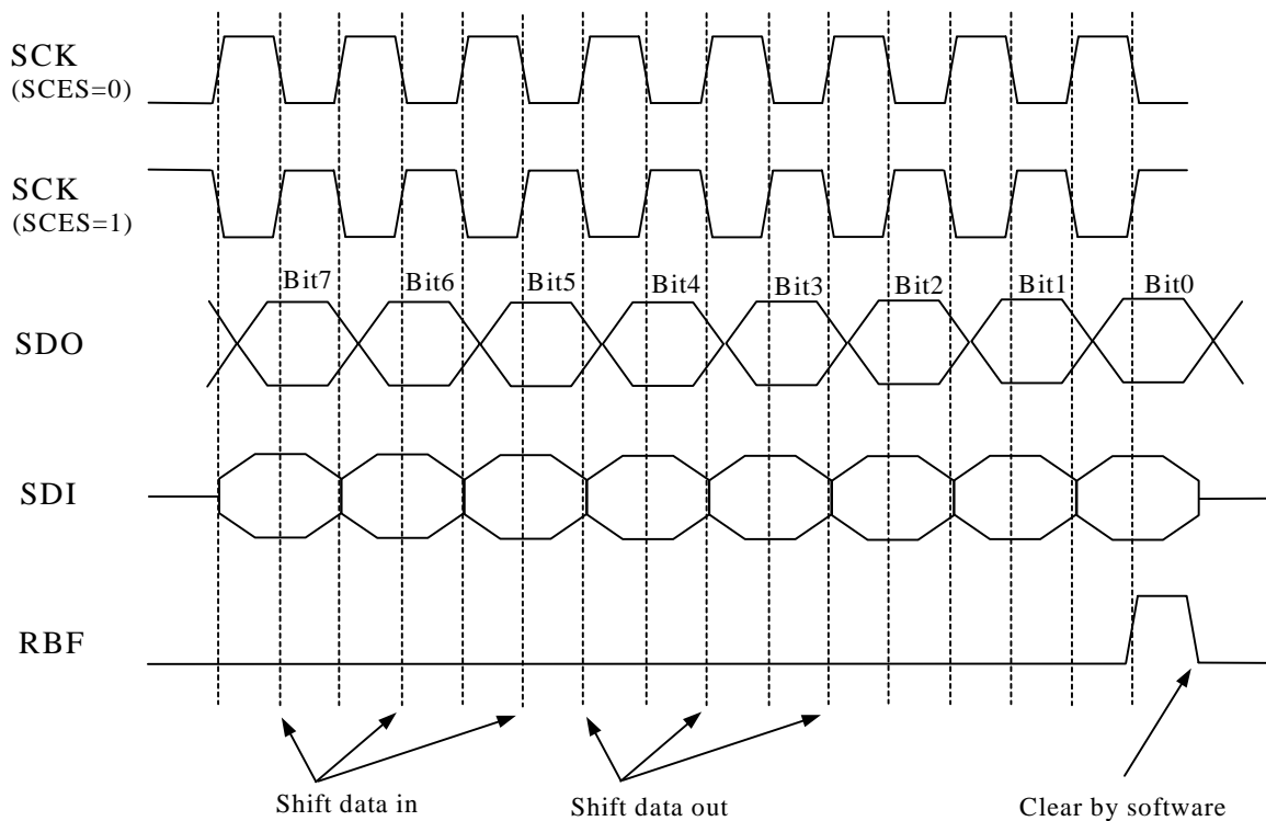
Fig. 14 SPI Timing
