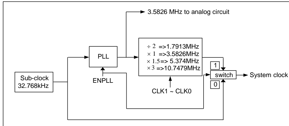
Fig. 18 Relationship between 32.768kHz and PLL
