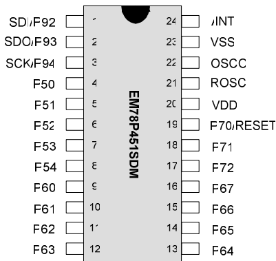
Figure 3-1c 24-pin SSOP EM78P451SDM
