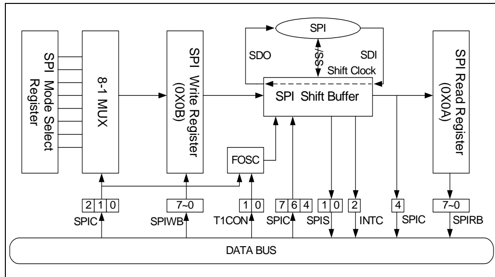
Figure 5-11 The Function Block Diagram of SPI Transmission
