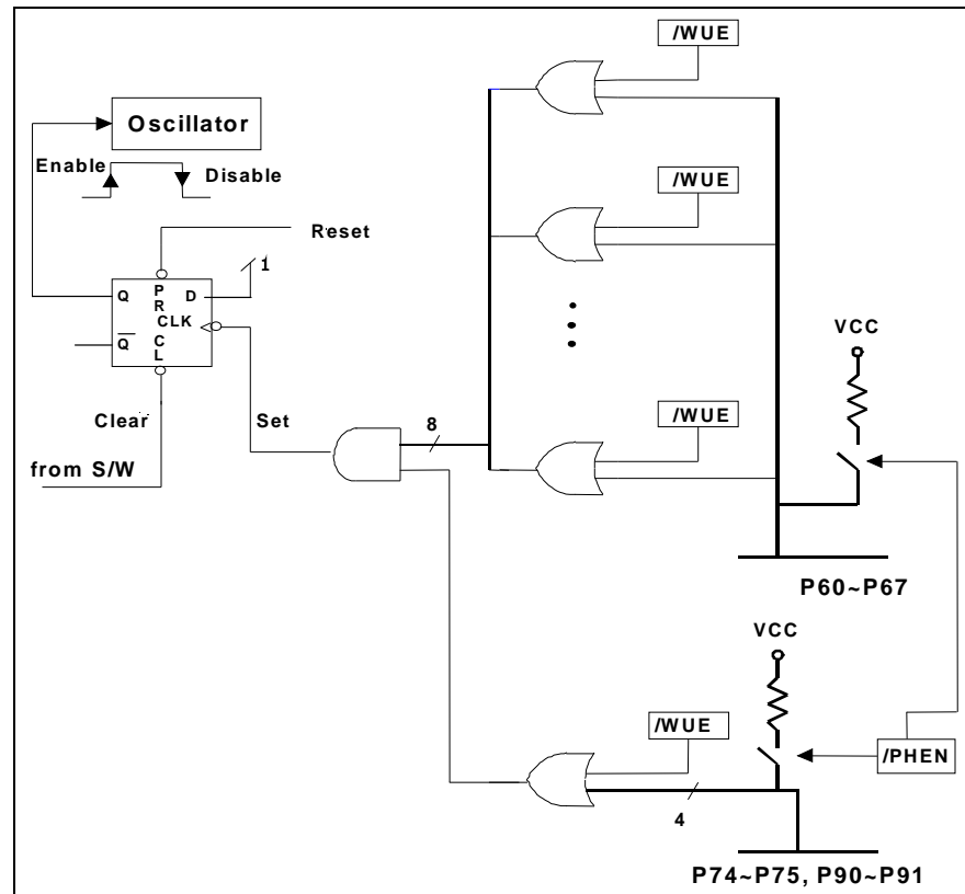
Figure 5-4 Block Diagram of Sleep Mode and Wake-up Circuits on I/O Ports
