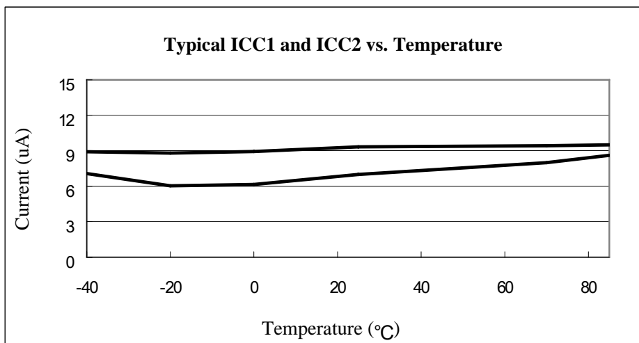
Fig. 6-10 Graph on Typical Operating Current (ICC1 and ICC2) vs. Temperature
