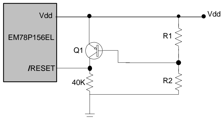
Fig. 16 Circuit 2 for the Residue Voltage Protection
