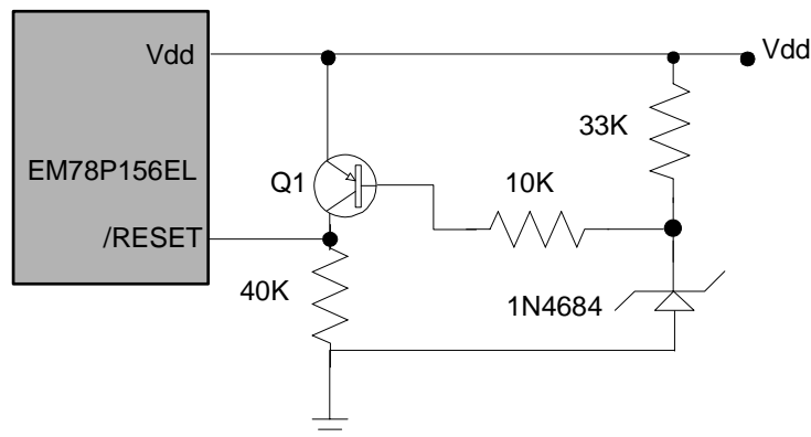
Fig. 15 Circuit 1 for the Residue Voltage Protection
