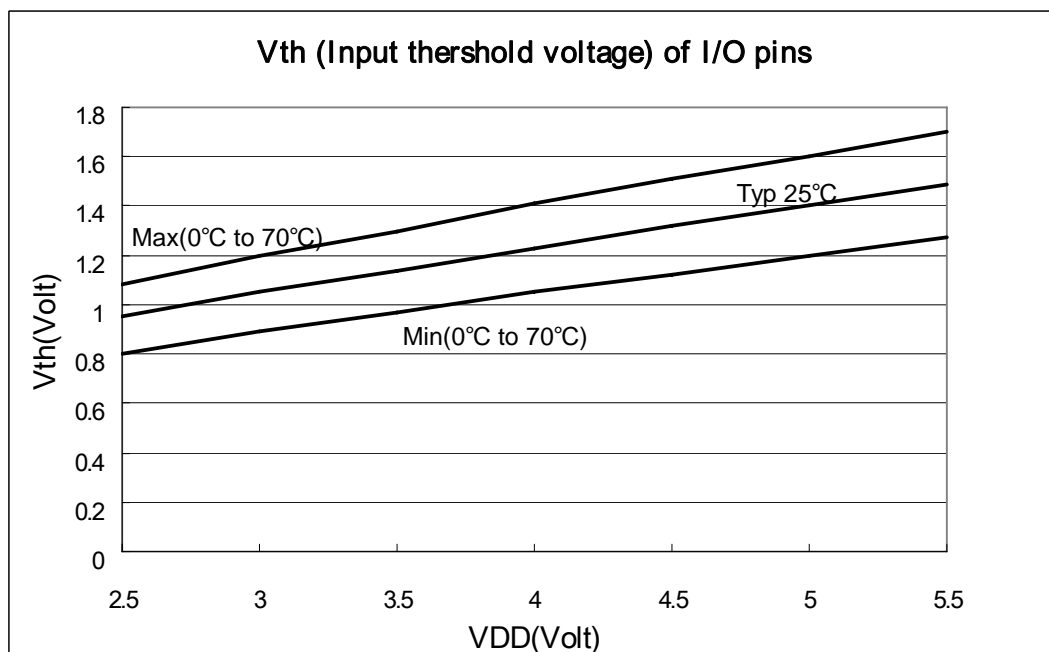
Fig. 18 Vth (Threshold voltage) of Port5 vs. VDD
