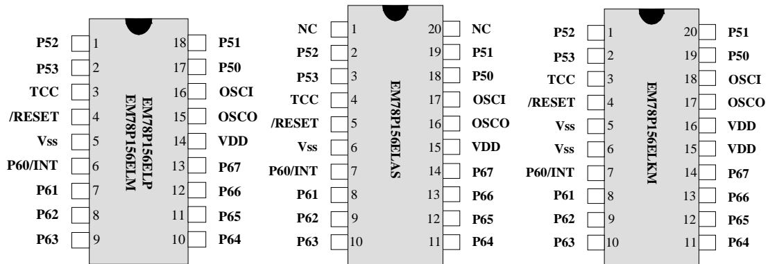
Fig. 1 Pin Assignment
