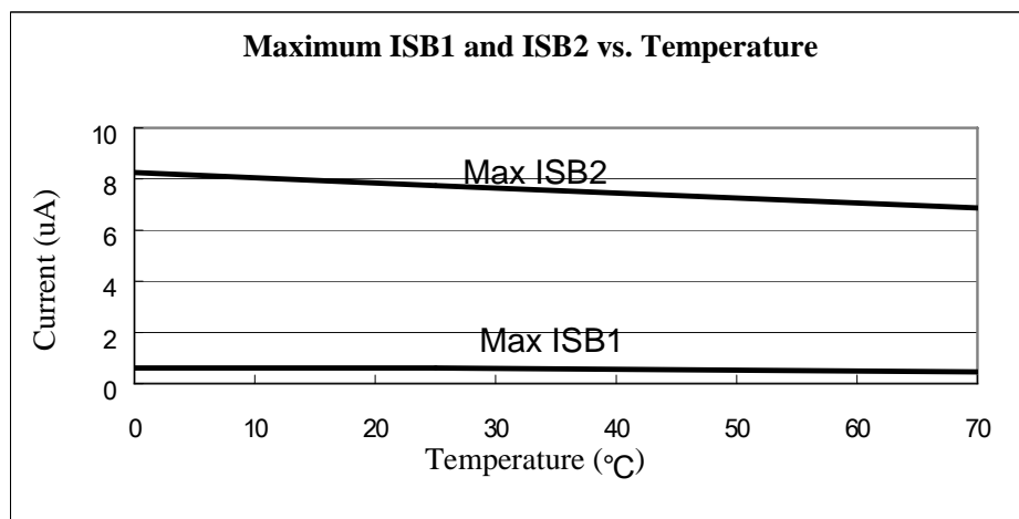
Fig. 31 Maximum standby current (ISB1 and ISB2) vs. Temperature
