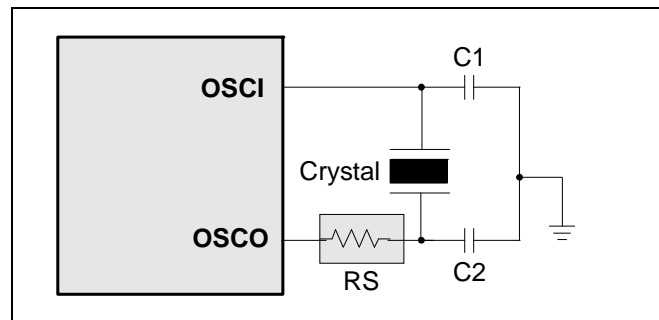
Figure 6-13 Crystal/Resonator Circuit
