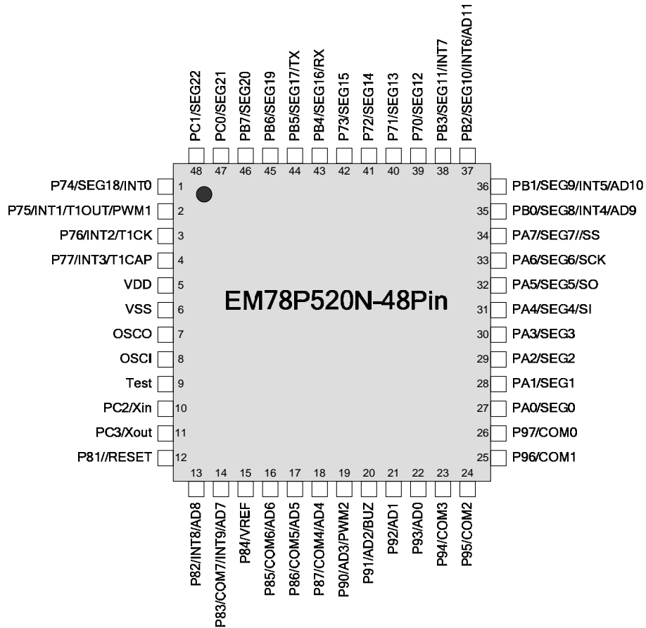
Figure 3-3 EM78P520NL48
