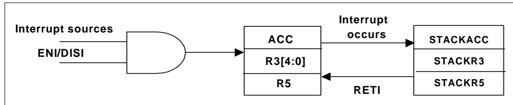
Figure 6-15 Interrupt Backup Diagram
