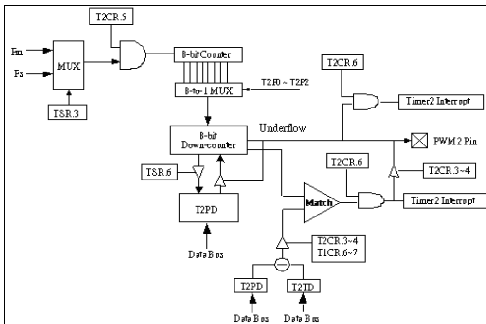
Figure 6-30 Timer 2 Configuration
