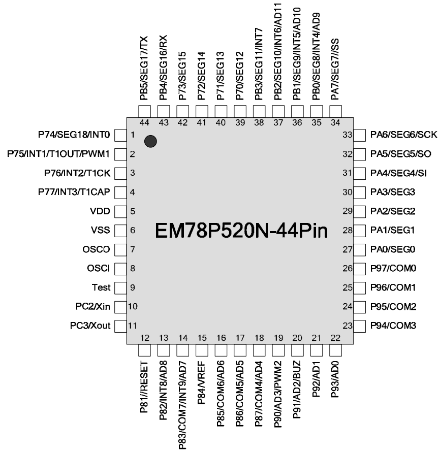
Figure 3-2 EM78P520NQ44/L44
