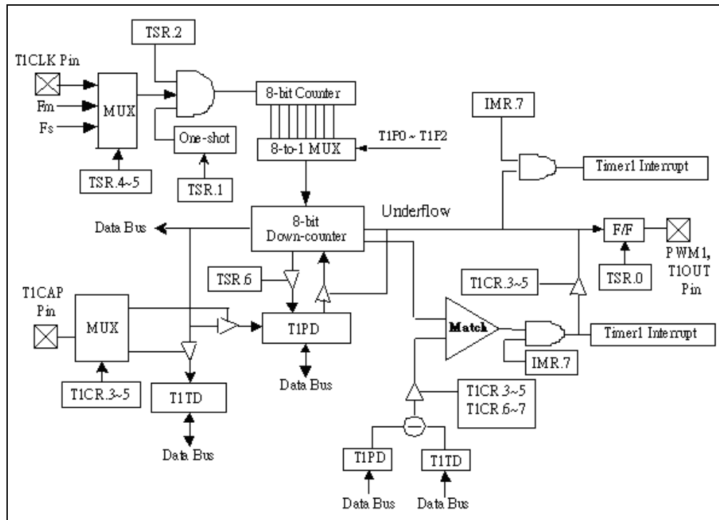
Figure 6-26 Timer/Counter 1 Configuration
