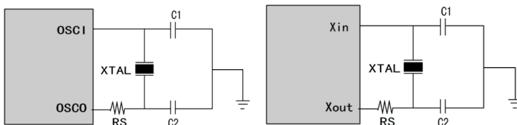
Figure 6-7-1 Circuit for Crystal/Resonator
