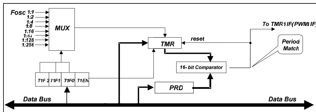
Figure 6-11 16-Bit Timer Functional Block Diagram (Merged from Two 8-Bit Timers)
