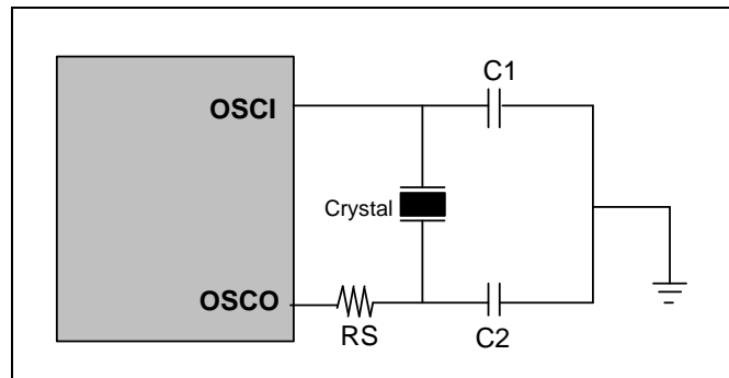
Figure 6-15b Crystal/Resonator Circuit
