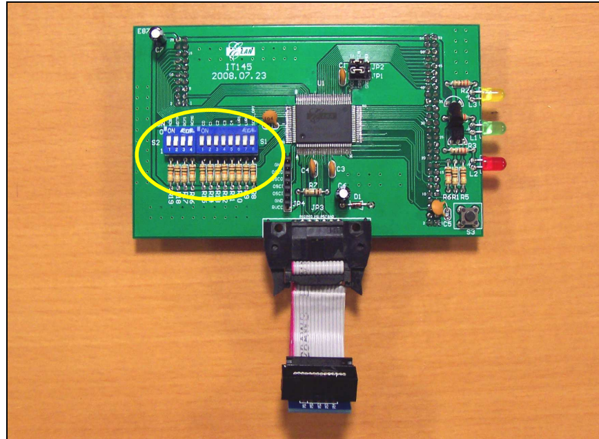
Figure C-2 ICE 143 Indicating DIP Switch Location
