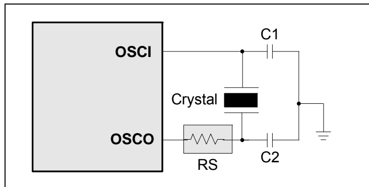
Figure 5-18 Crystal/Resonator Circuit
