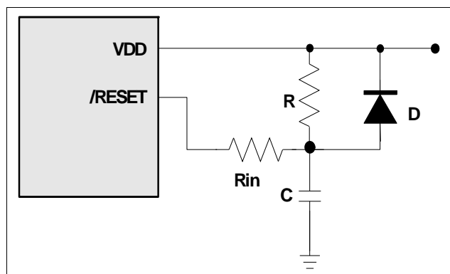
Figure 5-20 External Power-on Reset Circuit
