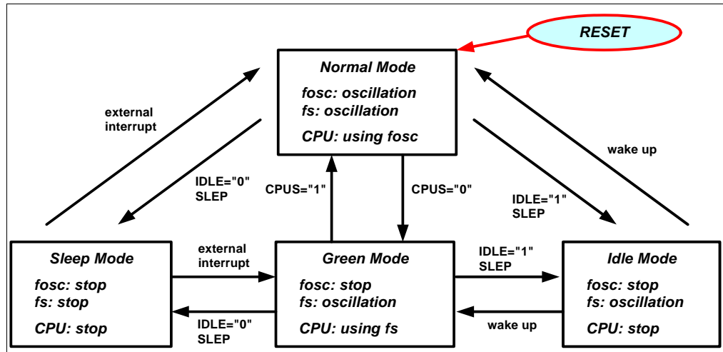
Figure 5-3 CPU Operation Mode
