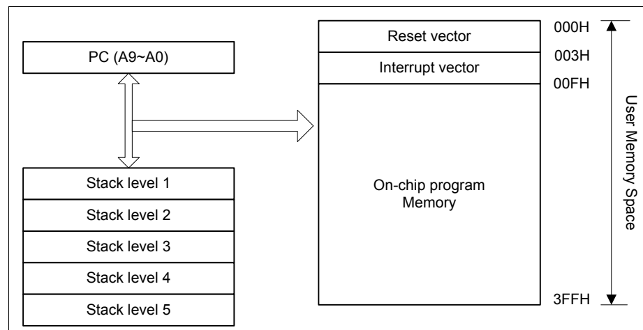
Figure 5-2 Program Counter Organization
