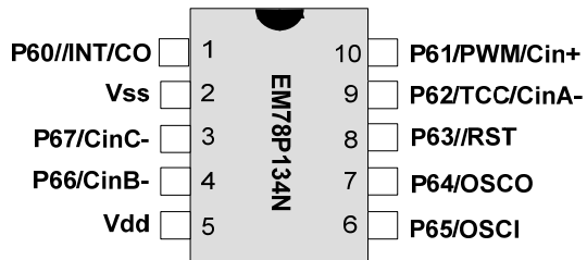
Figure 3-1 EM78P134NMS10J
