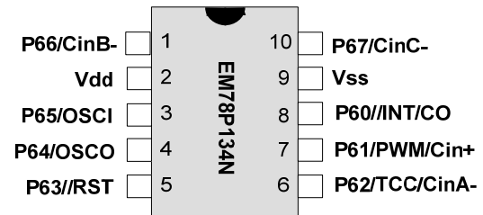
Figure 3-2 EM78P134NSS10 J
