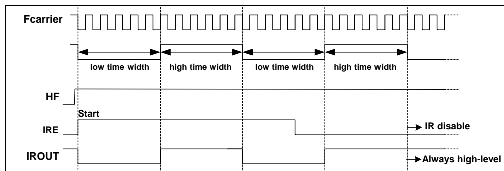
Figure 6-11d LGP=0, HF=0, When IRE goes Low from High, IROUT Pin Output Waveform
