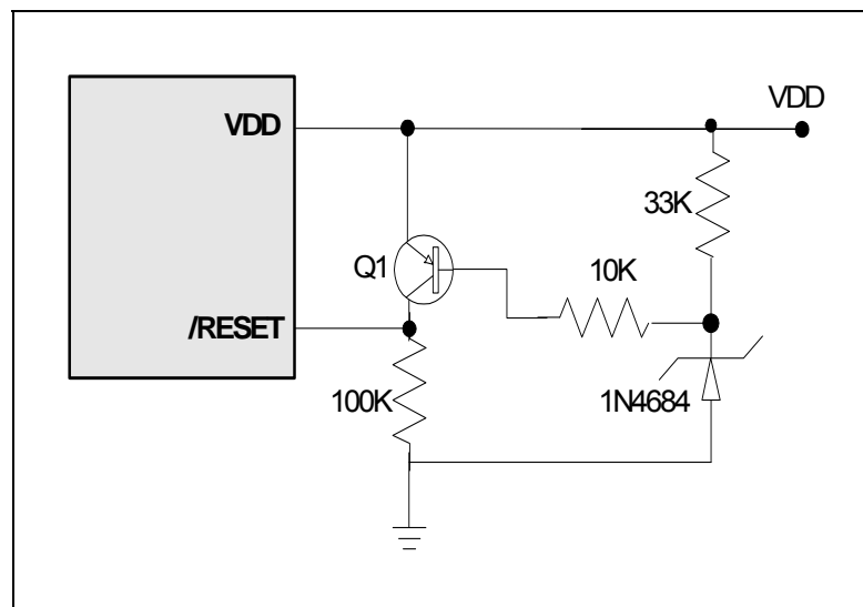
Figure 6-20 Residual Voltage Protection Circuit 1
