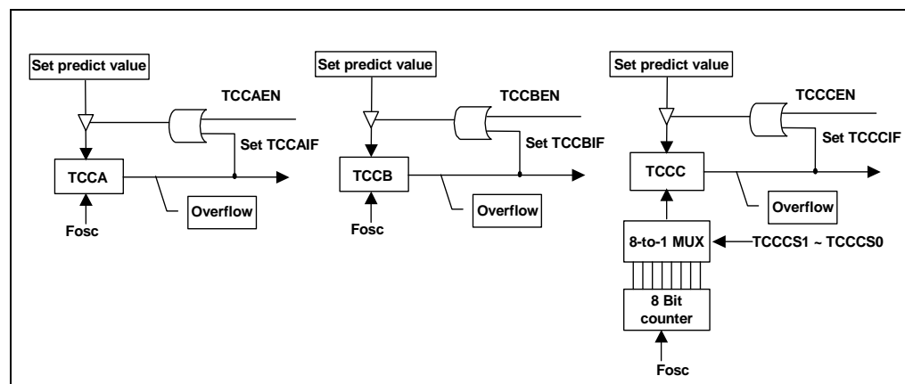
Figure 6-12 Timer Block Diagram
