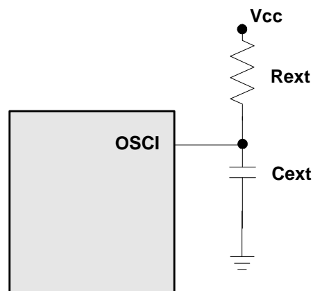
Figure 6-18 External RC Oscillator Mode Circuit
