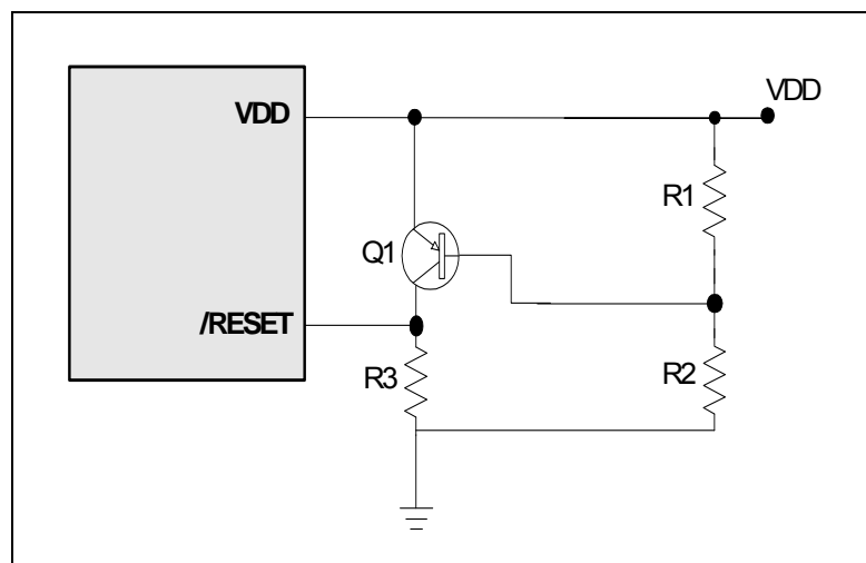
Figure 6-21 Residual Voltage Protection Circuit 2
