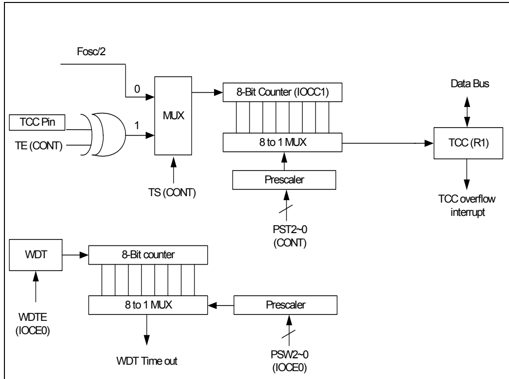
Figure 6-3 TCC and WDT Block Diagram
