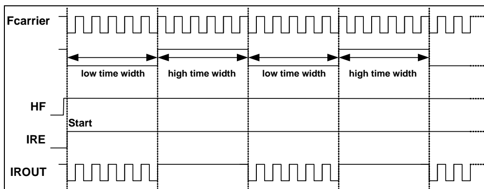
Figure 6-11a LGP=0, HF=1, IROUT Pin Output Waveform
