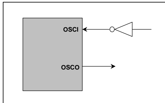
Figure 6-13 External Clock Input Circuit
