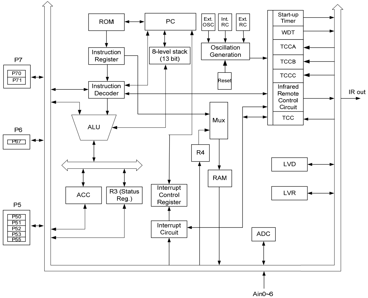
Figure 5 EM78P142 Block Diagram
