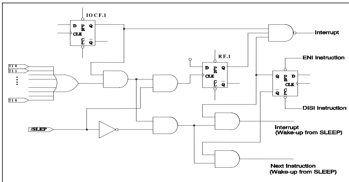
Figure 6-6 Port 5 Block Diagram with Input Change Interrupt/Wake-up
