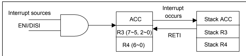
Figure 6-8 Interrupt Back-up Diagram
