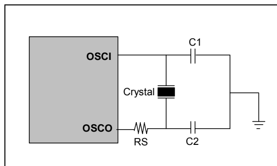
Figure 6-14 Crystal/Resonator Circuit
