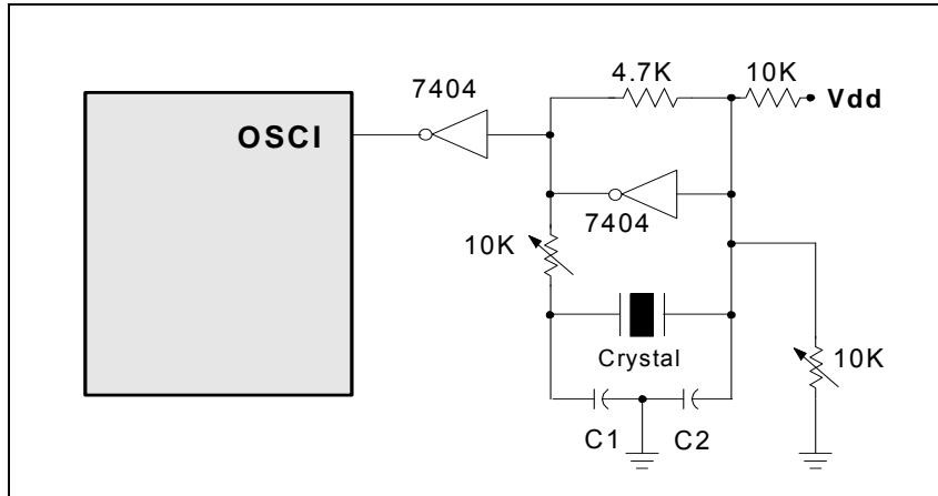
Figure 6-16 Parallel Mode Crystal/Resonator Circuit Diagram
