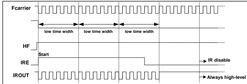
Figure 6-11e LGP=1 and HF=1, IROUT Pin Output Waveform
