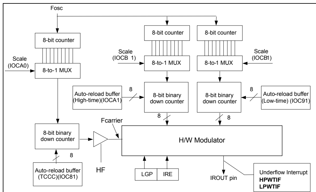
Figure 6-10 IR/PWM System Block Diagram
