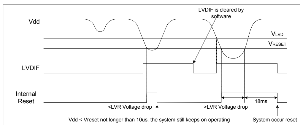
Figure 6-22 LVD/LVR Waveform Diagram
