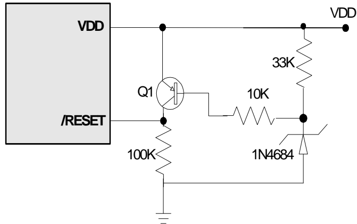
Figure 6-19 Residual Voltage Protection Circuit 1
