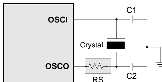
Figure 6-15 Crystal/Resonator Circuit
