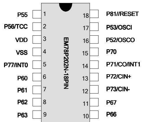
Figure 3-2 EM78P202ND18/SO18
