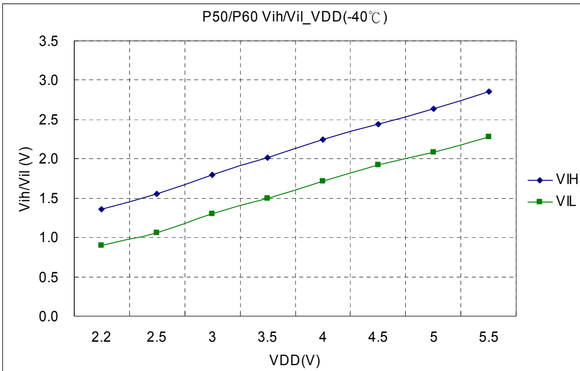
Figure 7-2 Vih, Vil vs. VDD (-40 °C)
