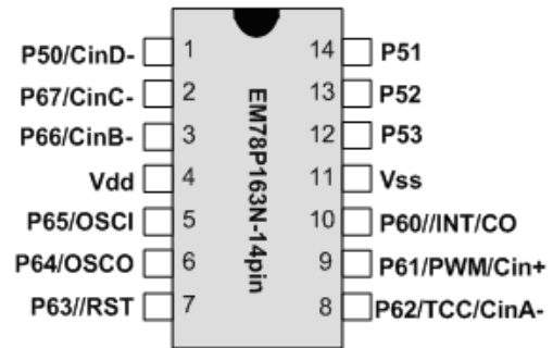
Figure 3-2 EM78P163ND14/SO14
