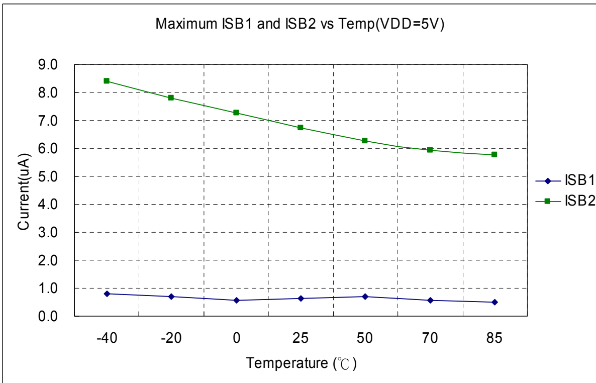
Figure 7-12 Maximum Standby Current (VDD=5V) vs. Temperature
