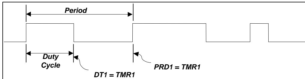
Figure 5-13 PWM Output Timing
