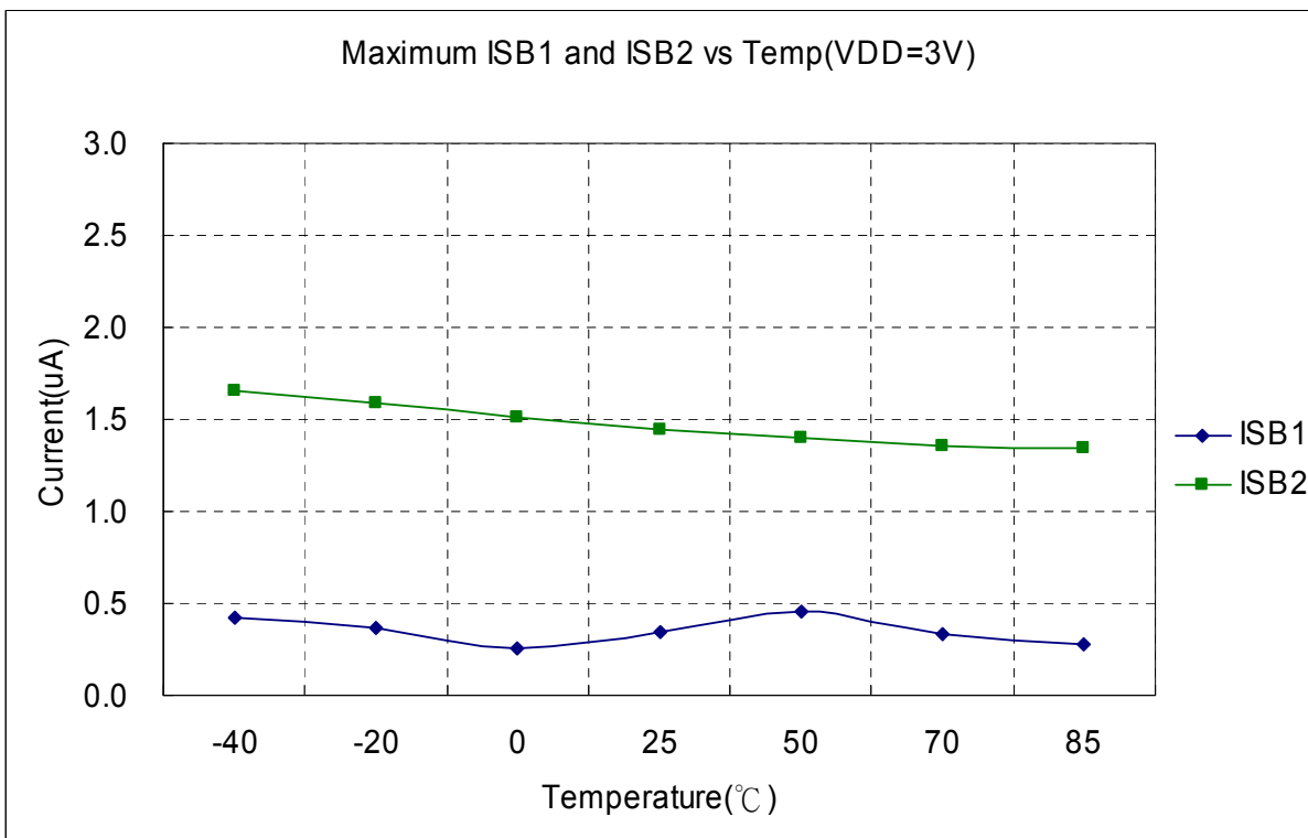
Figure 7-14 Maximum Standby Current (VDD=3V) vs. Temperature
