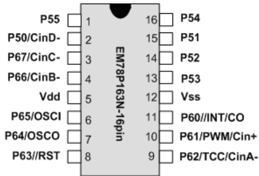
Figure 3-1 EM78P163ND16/SO16
