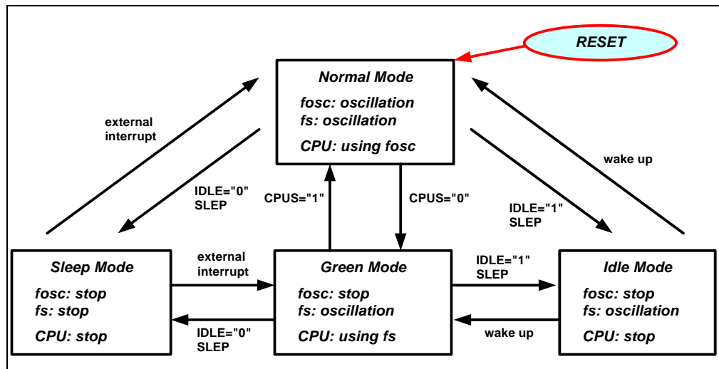
Figure 5-3 CPU Operation Mode
