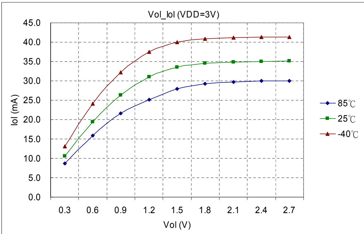
Figure 7-6 Vol vs. Iol at VDD=3V
