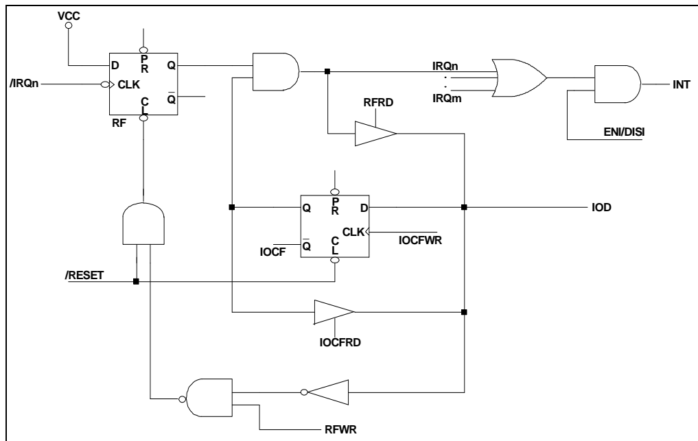
Figure 5-11 Interrupt input Circuit
