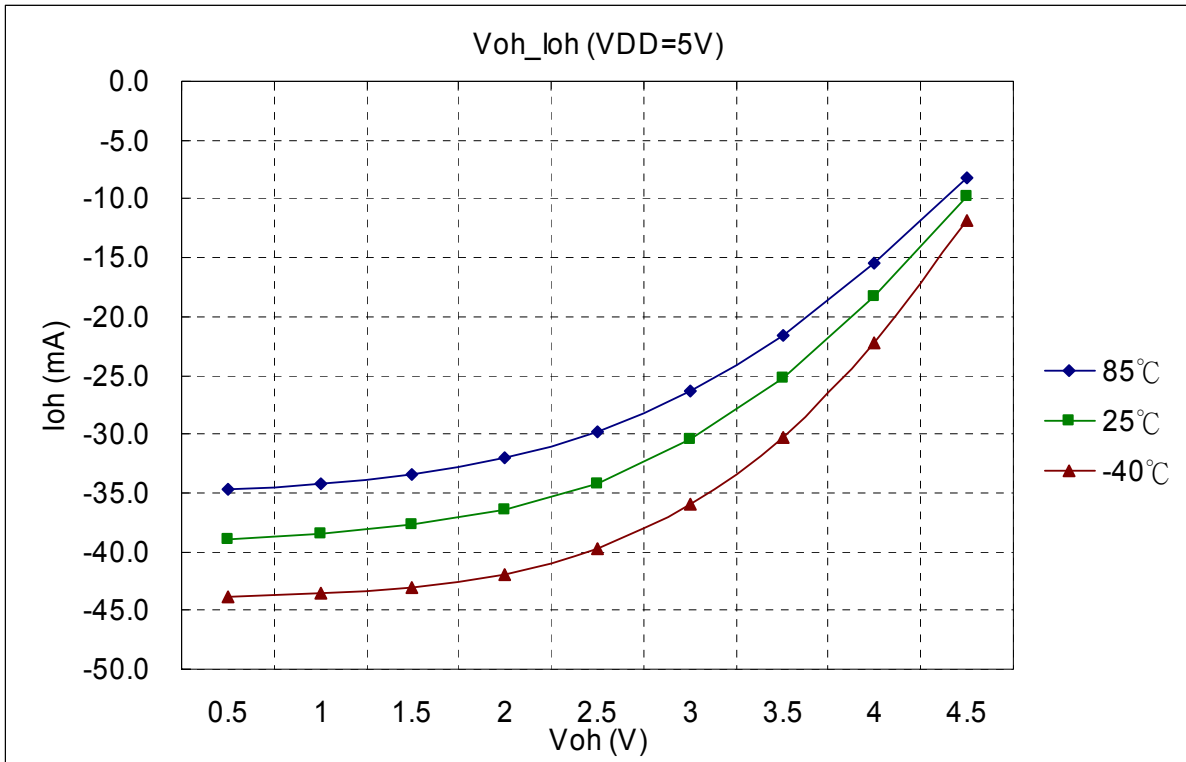
Figure 7-5 Voh vs. Ioh at VDD=5V
