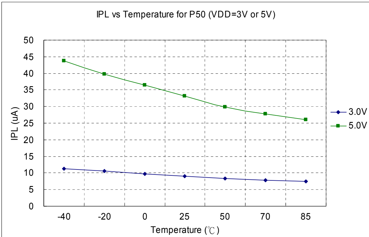
Figure 7-9 IPL vs. Temperature
