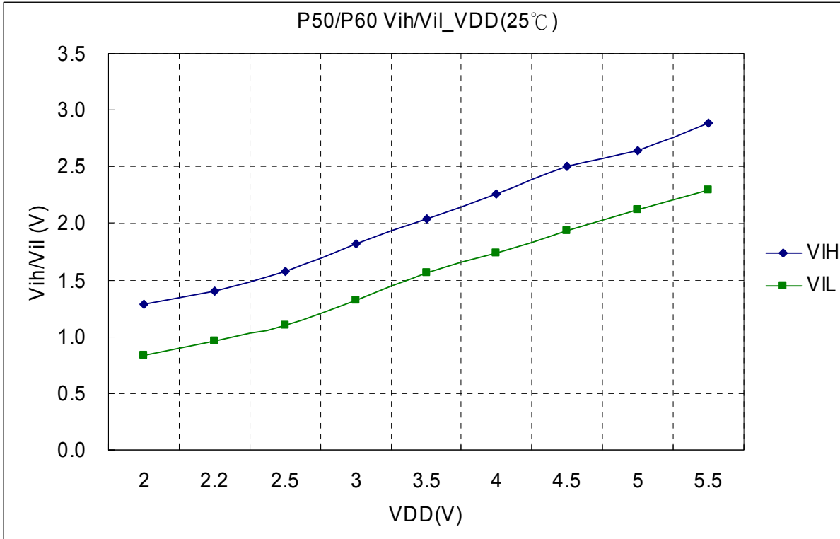
Figure 7-1 Vih, Vil vs. VDD (25°C)
