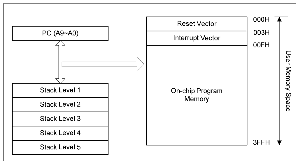
Figure 5-2 Program Counter Organization
