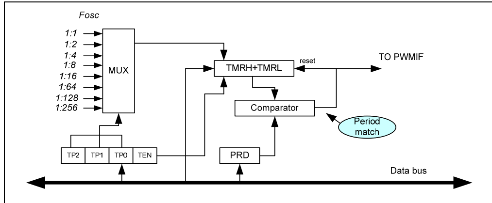
Figure 5-14 TMRX Block Diagram
