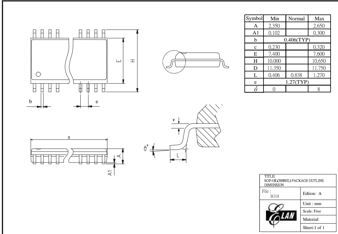
Figure B-1d EM78P156K 18-Lead SOP Package Type
