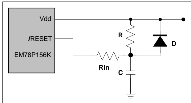
Figure 6-16 External Power-up Reset Circuit
