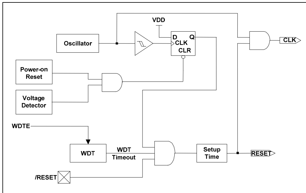
Figure 6-10 Controller Reset Block Diagram
