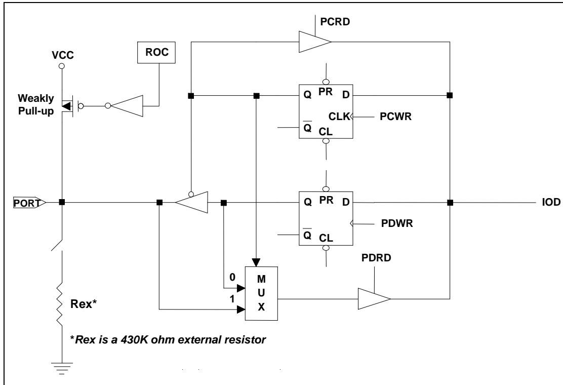
Figure 6-9 Circuit of I/O Port with R-Option (P50, P51)
