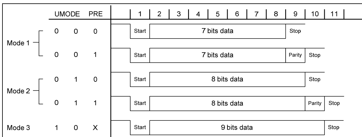
Figure 6-16 UART Model
