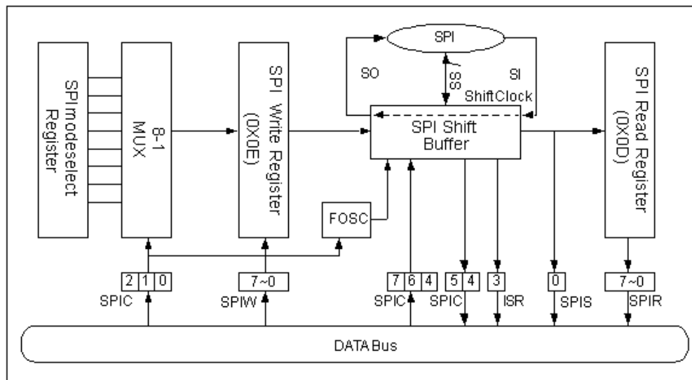
Figure 6-21 Functional Block Diagram of SPI Transmission
