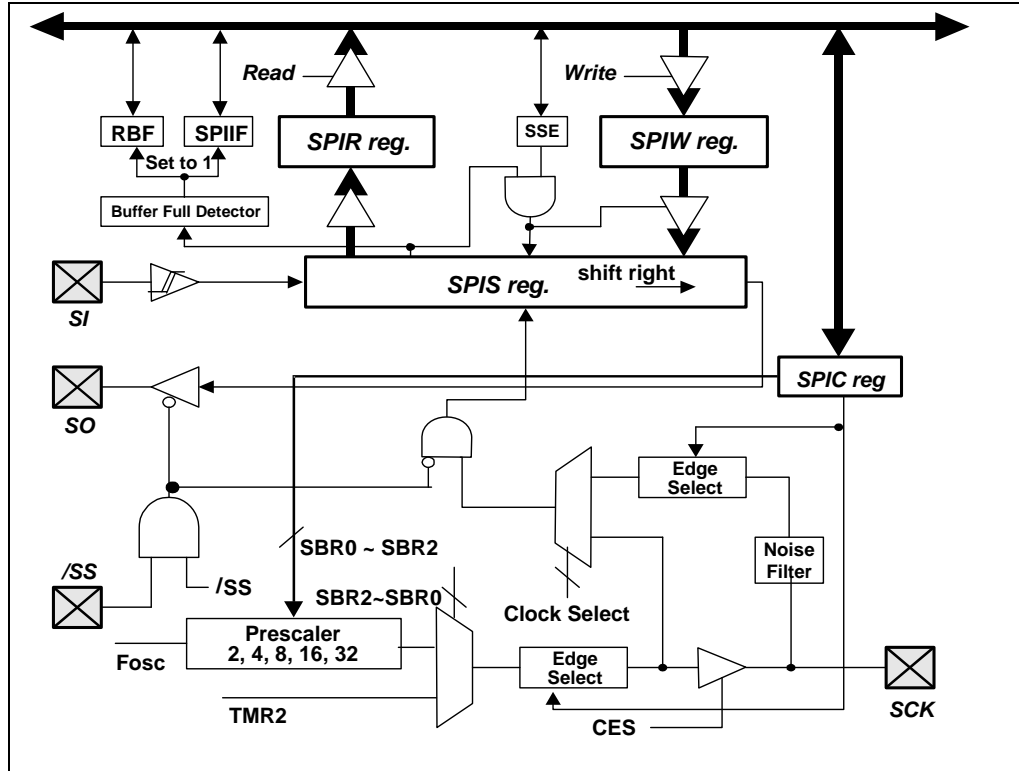
Figure 6-20 SPI Block Diagram
