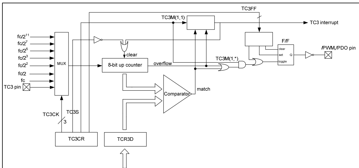
Figure 6-10 Timer/Counter 3 Configuration
