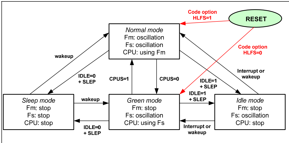
Figure 6-3 CPU Operation Mode
