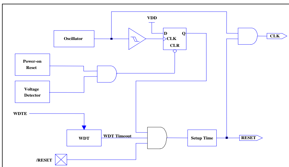
Figure 6-38 Block Diagram of Controller Reset
