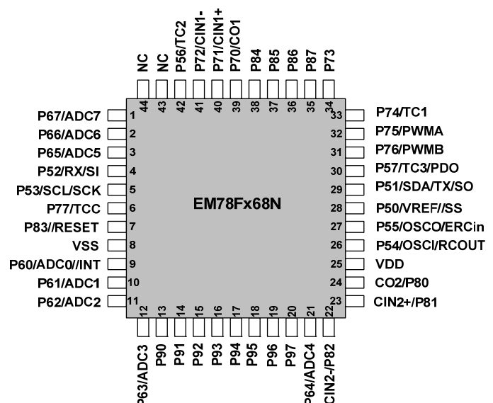
Figure 3-4 40-pin EM78Fx68N
