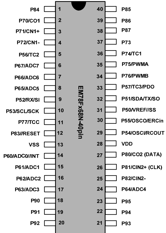
Figure 3-2 40-pin EM78Fx68N
