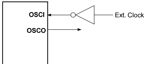
Figure 6-42 External Clock Input Circuit
