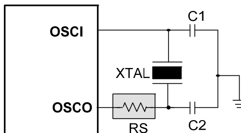
Figure 6-43 Crystal/Resonator Circuit
