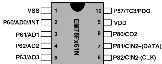
Figure 3-1a EM78F61NMS10
