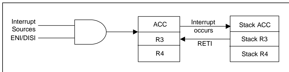
Figure 6-13 Interrupt Back-up Diagram
