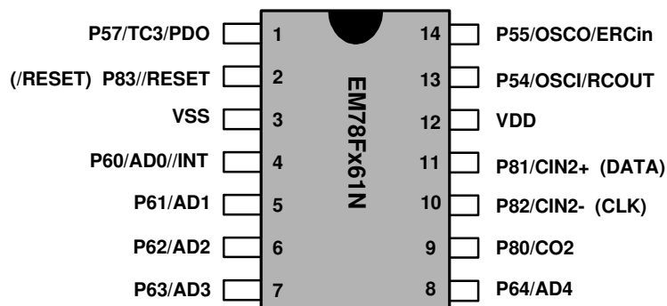
Figure 3-1c EM78F61NSO14
