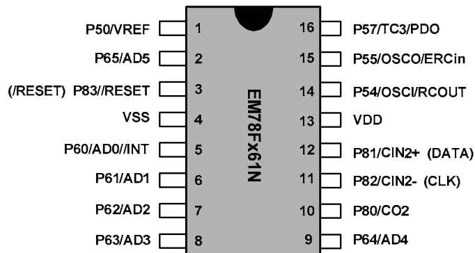
Figure 3-1b EM78F61NAD16 / EM78F61NASO16A
