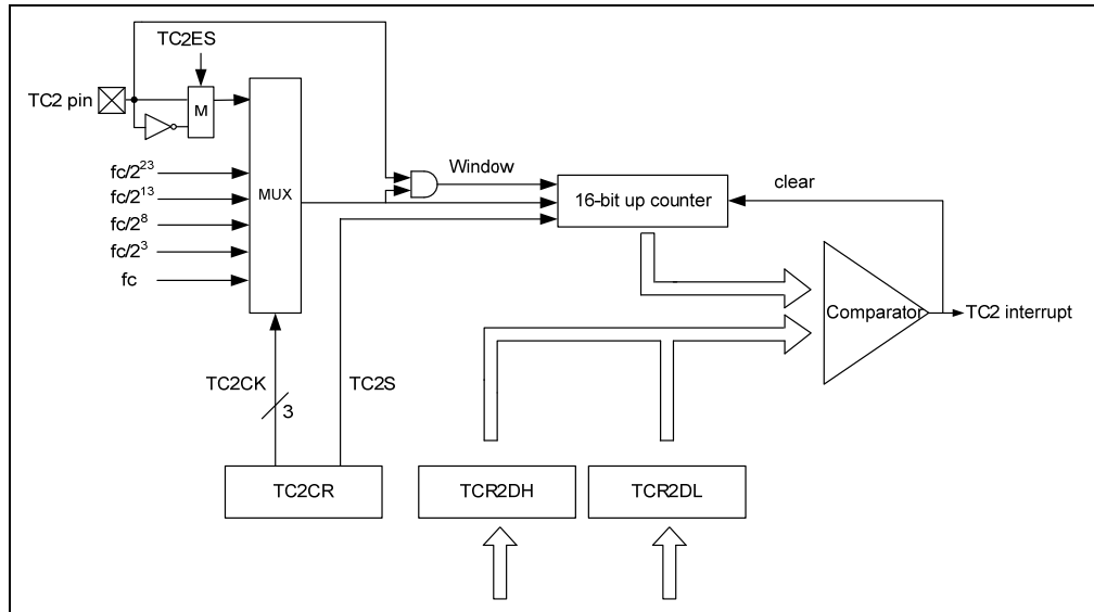
Figure 6-9a Timer/Counter 2 Configuration Block Diagram
