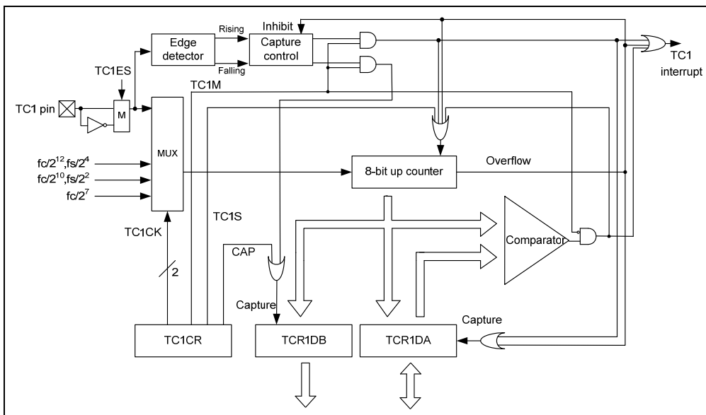
Figure 6-8a Timer/Counter 1 Configuration Block Diagram
