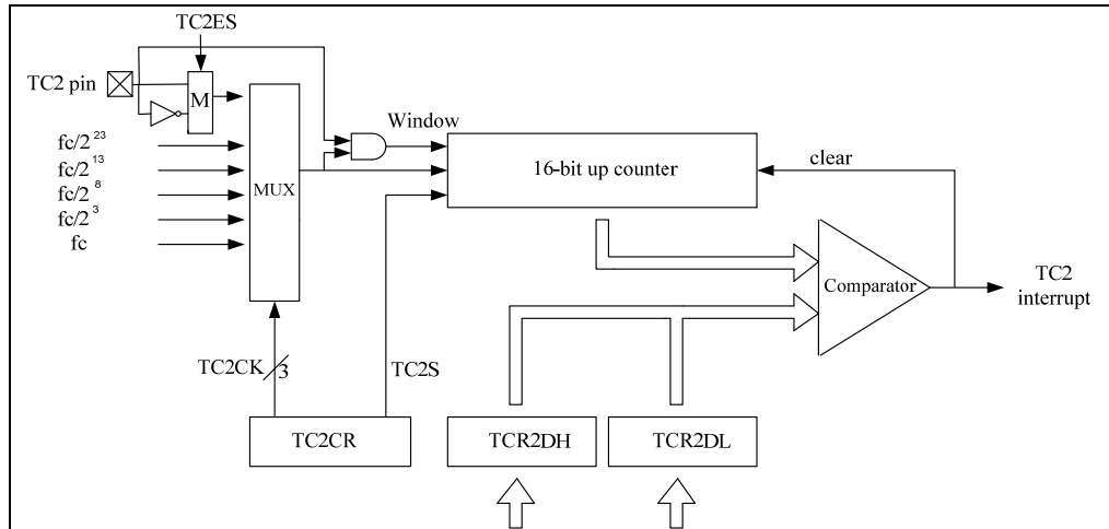
Figure 6-4a Timer/Counter 2 Configuration Block Diagram
