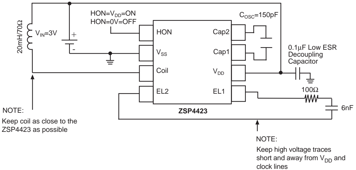
Figure 3. Test Circuit
