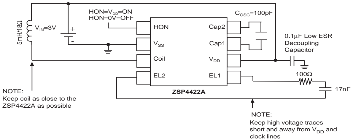
Figure 3. Test Circuit
