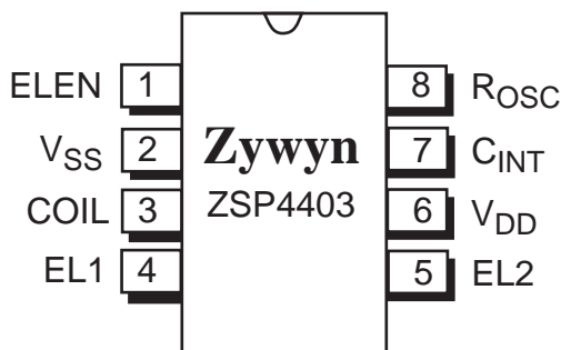
8-Pin MSOP
