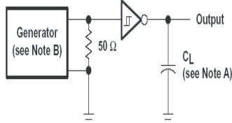
TEST CIRCUIT
