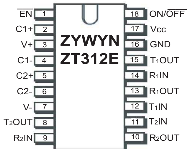
18-pin PDIP/wSOIC
