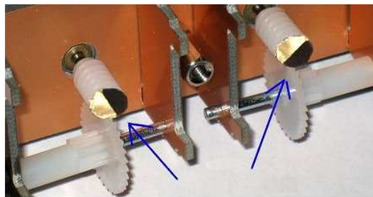
Fig 6 The black and silver discs form the wheel counters and should be as close to half and half as possible, to ensure the counts are as even.
