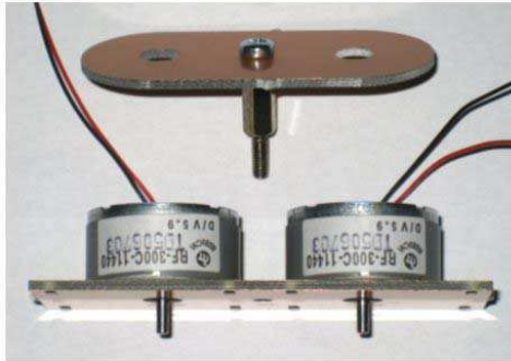
Fig 2 Note the worm gears are not pushed tight against the motors allow about a 3mm gap.
