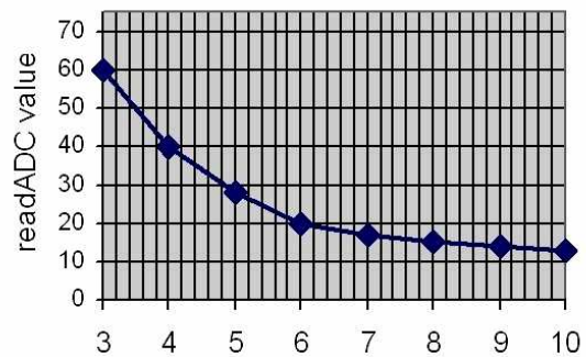
Approx ADC values for distance
