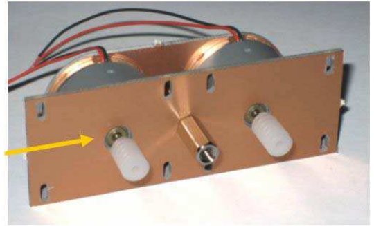
Fig 2 Note the worm gears are not pushed tight against the motors allow about a 3mm gap.
