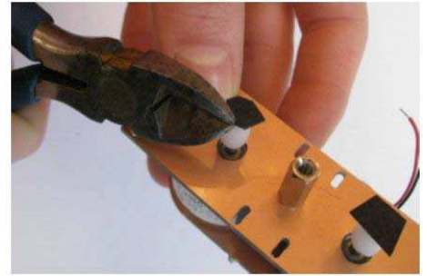
Fig4 A small piece of black card is secured using a contact adhesive. Be careful not to get any glue on the teeth of the worm gear. Once the glue has dried carefully trim the card to the same width as the gear.
