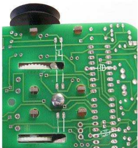
Fig 6 The black and silver discs form the wheel counters and should be as close to half and half as possible, to ensure the counts are as even.
