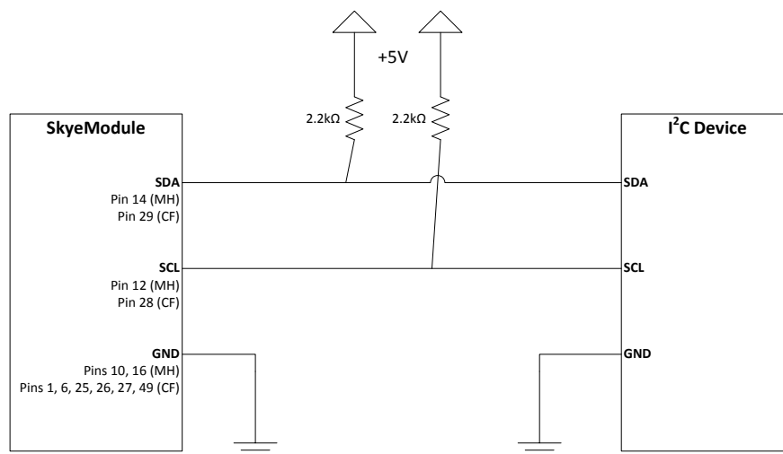
Figure 9-7 I2C Connection Diagram
