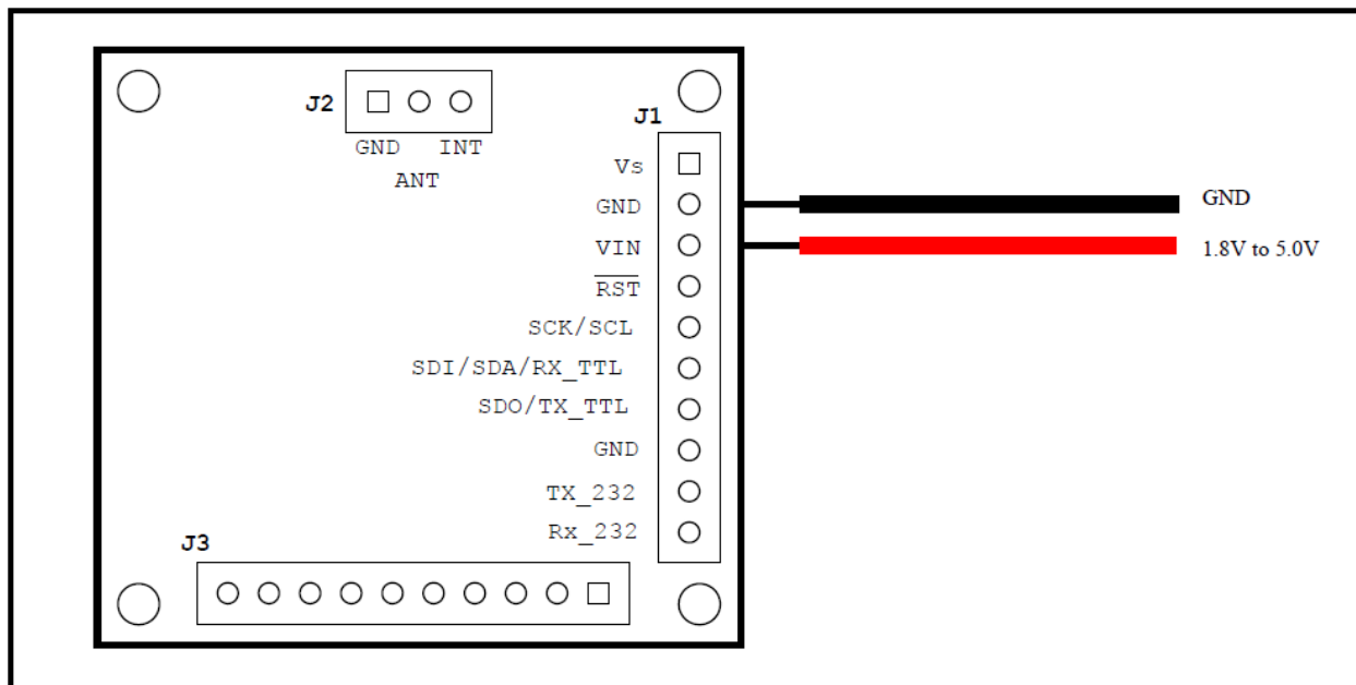
Figure 8-1: SkyeModule M1 Powered at V_{IN} \leq 5V
