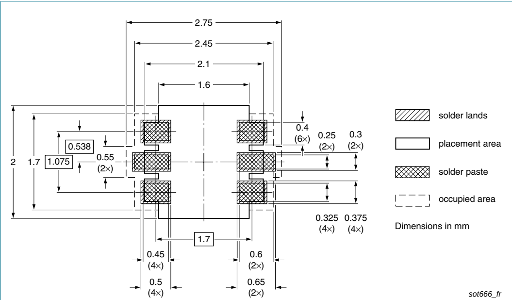
Fig 19. Reflow soldering footprint SOT666
