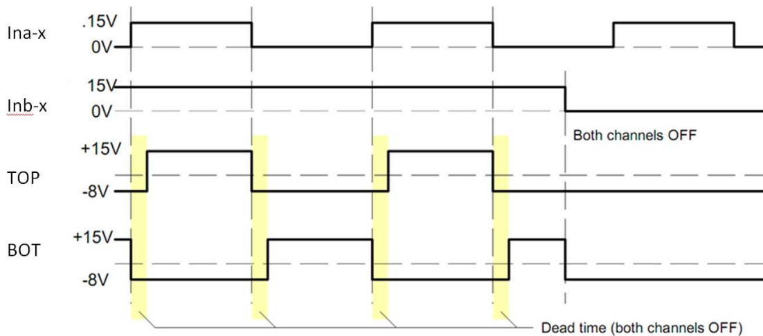
HB mode with dead time generation
