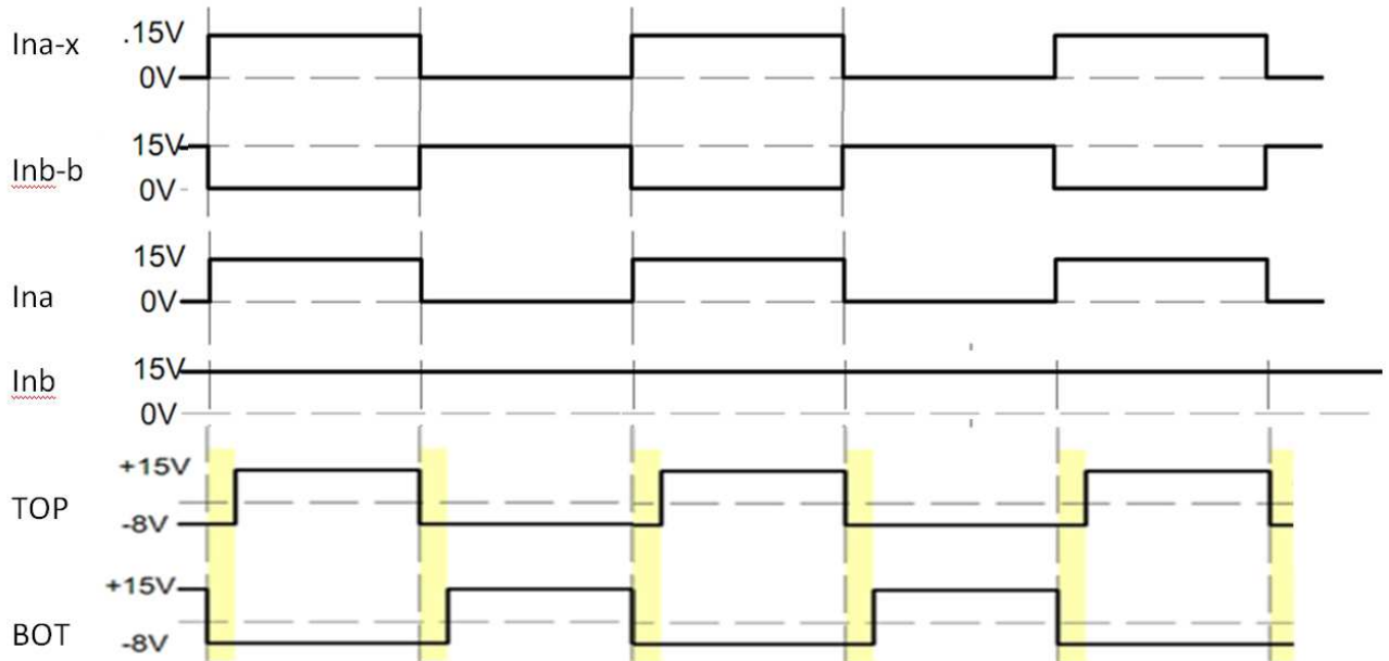
Input and output Signals with TOP-BOT configuration
