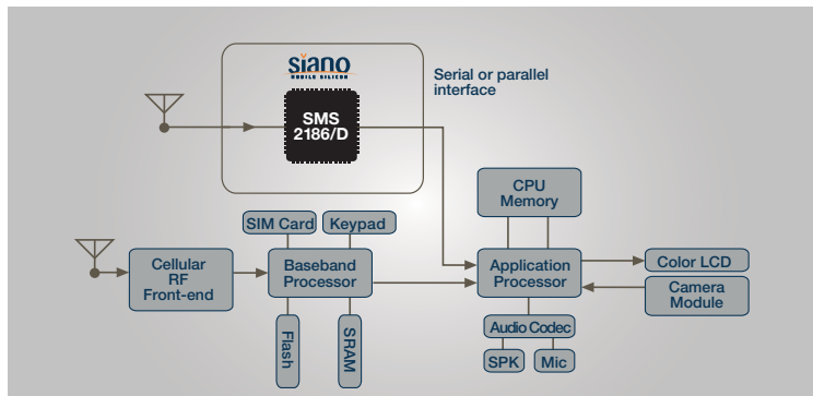
Integration of SMS2186/SMS2186D into a Mobile Device
