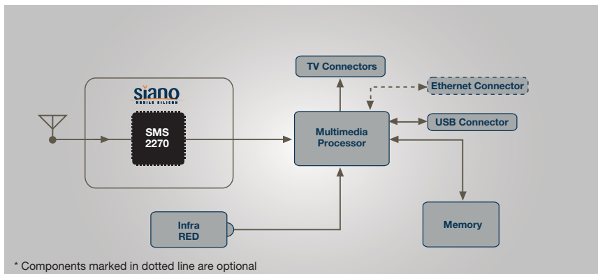
Integration of SMS2270 into a Set Top Box
