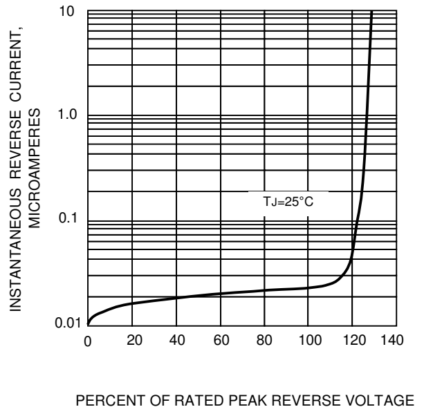
FIG.4-TYPICAL REVERSE CHARACTERISTICS
