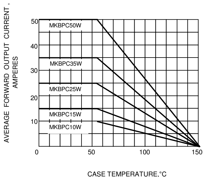
FIG.2- DERATING CURVE OUTPUT RECTIFIED CURRENT
