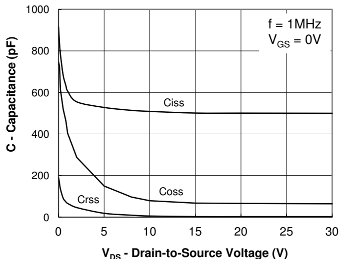
Fig.5 Capacitance Characteristic
