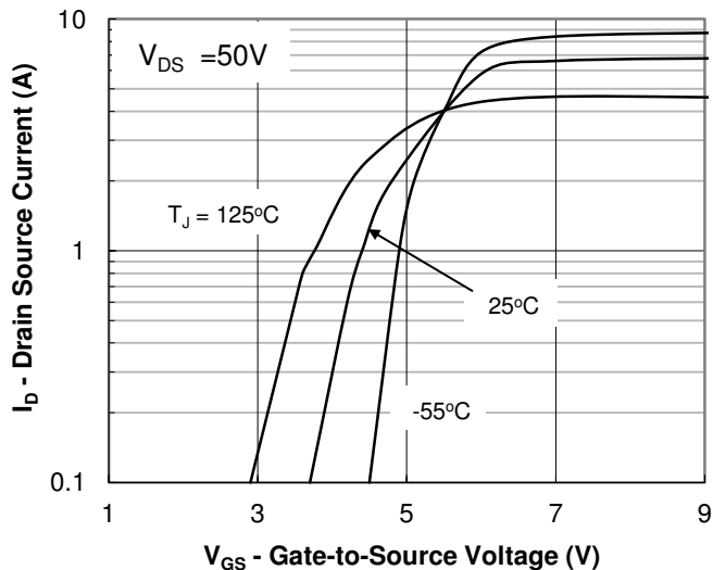
Fig.2 Transfer Characteristic
