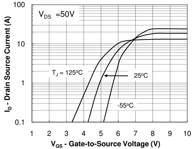
Fig.2 Transfer Characteristic
