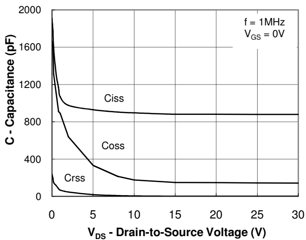
Fig.5 Capacitance Characteristic
