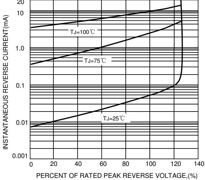
FIG.5-TYPICAL REVER CHARACTERISTICS
