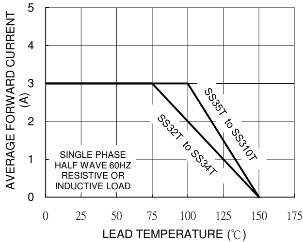
FIG.1 - FORWARD CURRENT RERATING CURVE
